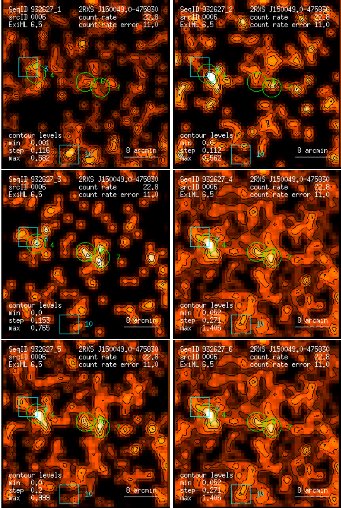
Figure 6: RASS 932627: detection 0006: band rate images, Gaussian filter: (1) PSPC channels 11 – 41, (2) 52 – 90, (3) 91 – 201, (4) 11 – 235, (5) 52 – 201, (6) 11 – 201. Broad band rates in counts/ks. Band rate contour levels in counts/ks/arcmin 2 .
