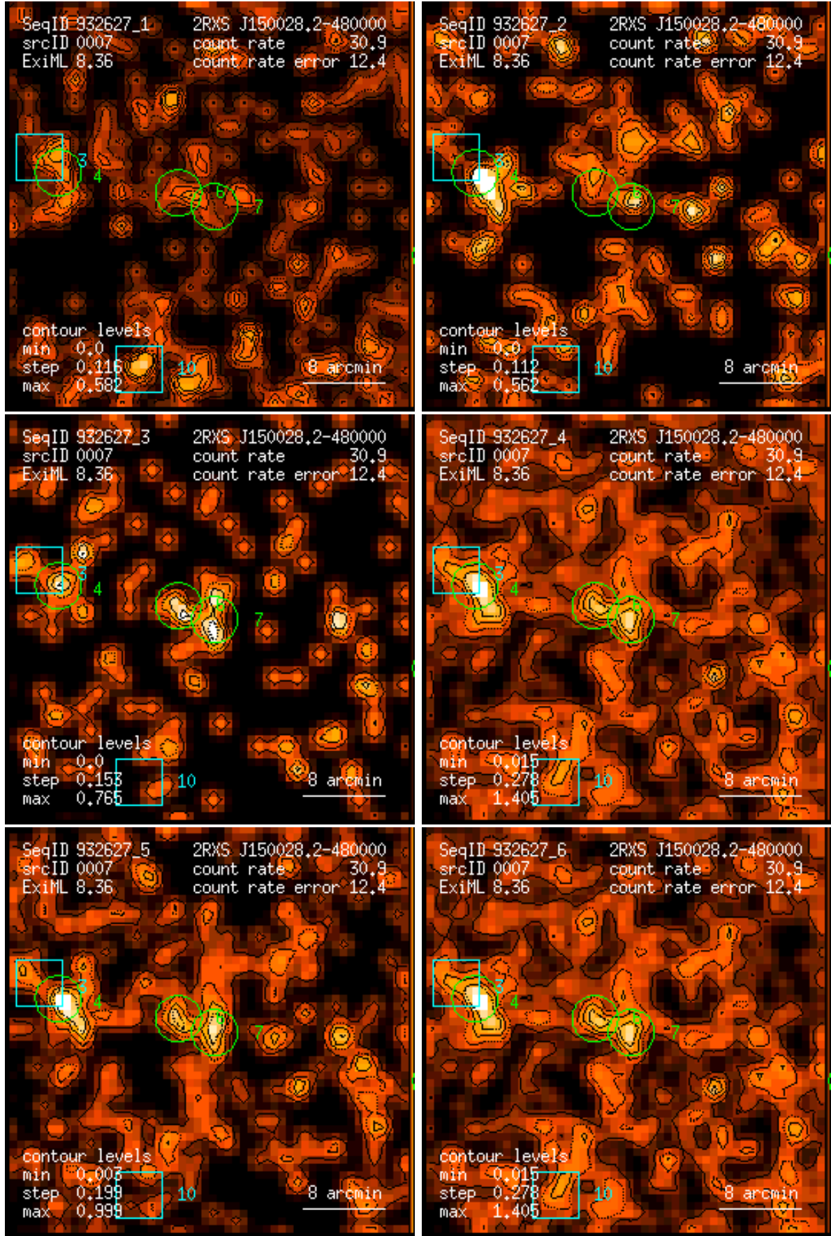
Figure 7: RASS 932627: detection 0007: band rate images, Gaussian filter: (1) PSPC channels 11 – 41, (2) 52 – 90, (3) 91 – 201, (4) 11 – 235, (5) 52 – 201, (6) 11 – 201. Broad band rates in counts/ks. Band rate contour levels in counts/ks/arcmin 2 .
