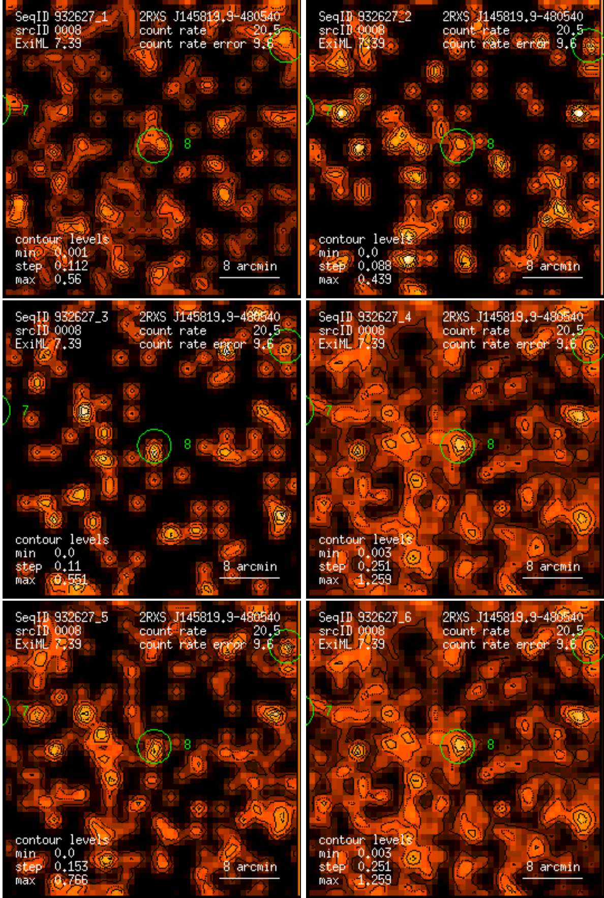
Figure 8: RASS 932627: detection 0008: band rate images, Gaussian filter: (1) PSPC channels 11 – 41, (2) 52 – 90, (3) 91 – 201, (4) 11 – 235, (5) 52 – 201, (6) 11 – 201. Broad band rates in counts/ks. Band rate contour levels in counts/ks/arcmin 2 .
