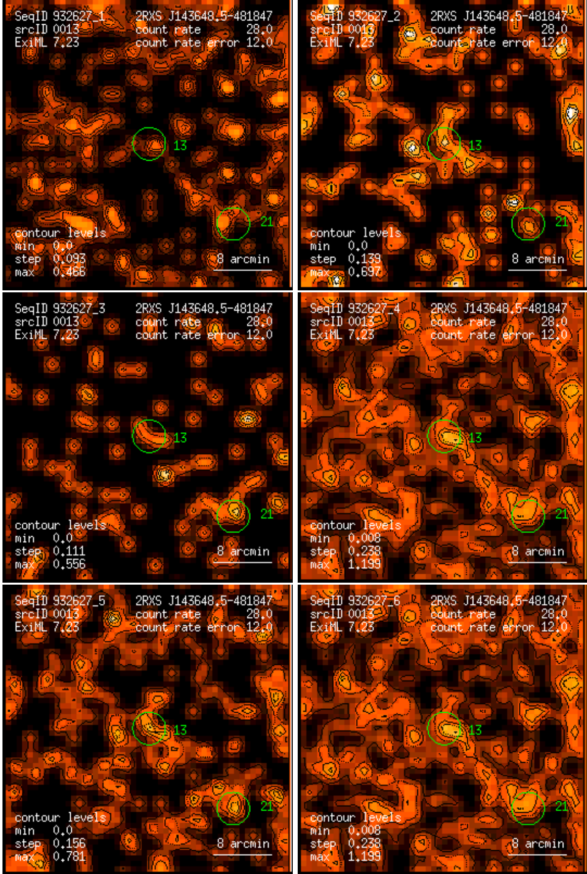
Figure 13: RASS 932627: detection 0013: band rate images, Gaussian filter: (1) PSPC channels 11 – 41, (2) 52 – 90, (3) 91 – 201, (4) 11 – 235, (5) 52 – 201, (6) 11 – 201. Broad band rates in counts/ks. Band rate contour levels in counts/ks/arcmin 2 .
