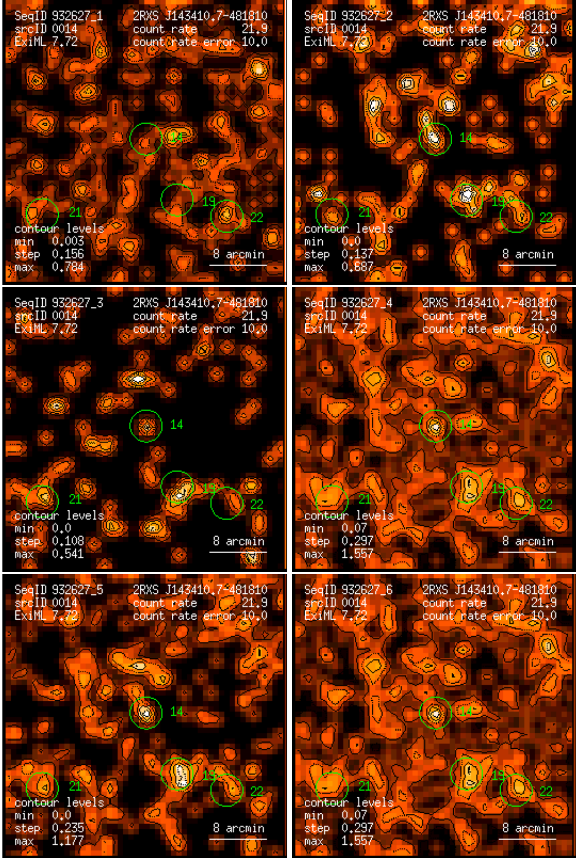
Figure 14: RASS 932627: detection 0014: band rate images, Gaussian filter: (1) PSPC channels 11 – 41, (2) 52 – 90, (3) 91 – 201, (4) 11 – 235, (5) 52 – 201, (6) 11 – 201. Broad band rates in counts/ks. Band rate contour levels in counts/ks/arcmin 2 .
