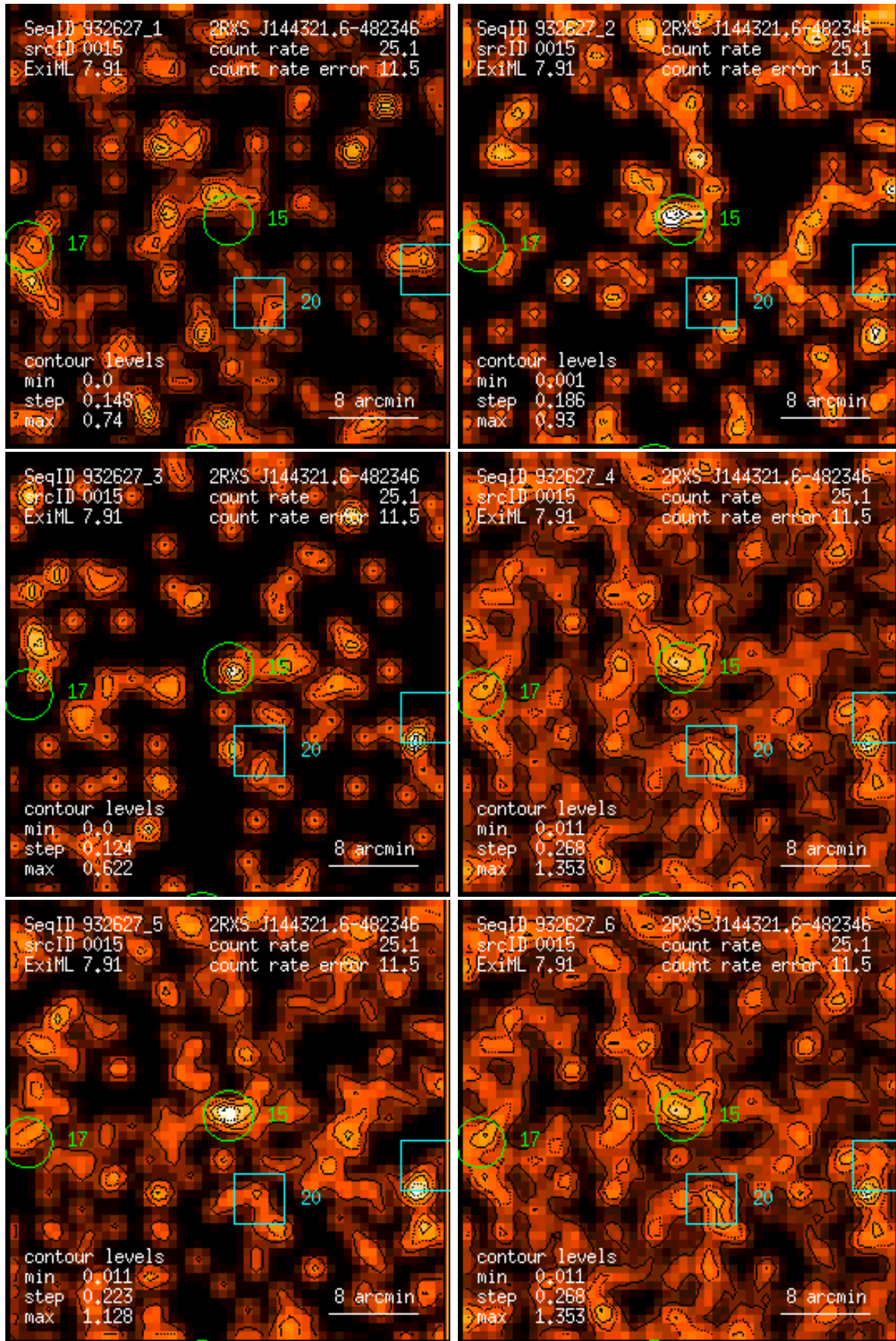
Figure 15: RASS 932627: detection 0015: band rate images, Gaussian filter: (1) PSPC channels 11 – 41, (2) 52 – 90, (3) 91 – 201, (4) 11 – 235, (5) 52 – 201, (6) 11 – 201. Broad band rates in counts/ks. Band rate contour levels in counts/ks/arcmin 2 .
