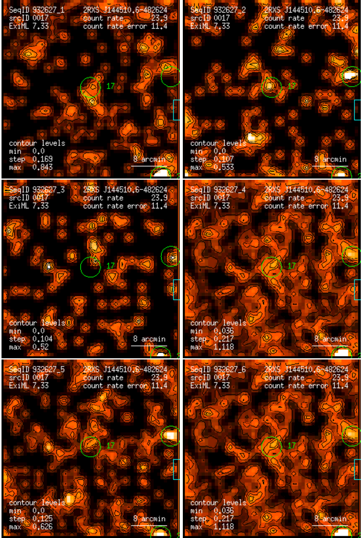
Figure 17: RASS 932627: detection 0017: band rate images, Gaussian filter: (1) PSPC channels 11 – 41, (2) 52 – 90, (3) 91 – 201, (4) 11 – 235, (5) 52 – 201, (6) 11 – 201. Broad band rates in counts/ks. Band rate contour levels in counts/ks/arcmin 2 .
