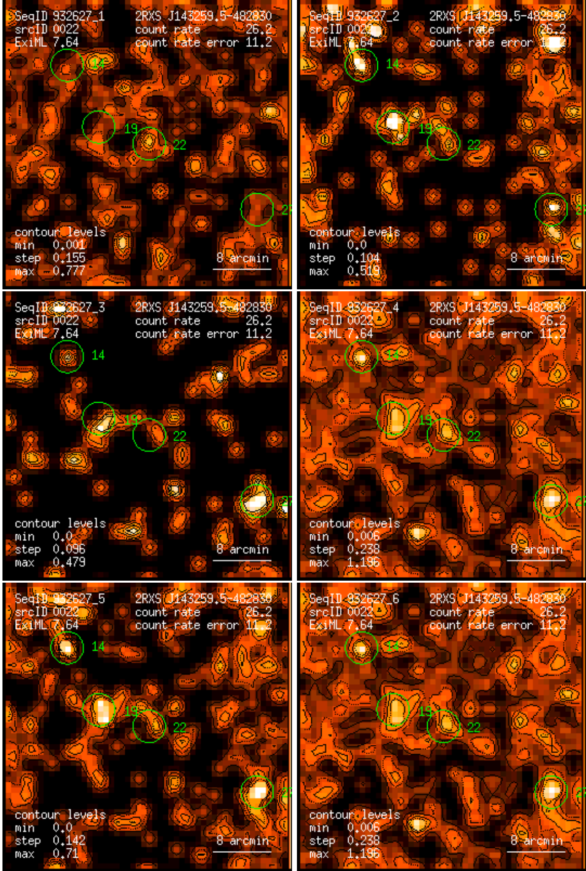
Figure 22: RASS 932627: detection 0022: band rate images, Gaussian filter: (1) PSPC channels 11 – 41, (2) 52 – 90, (3) 91 – 201, (4) 11 – 235, (5) 52 – 201, (6) 11 – 201. Broad band rates in counts/ks. Band rate contour levels in counts/ks/arcmin 2 .
