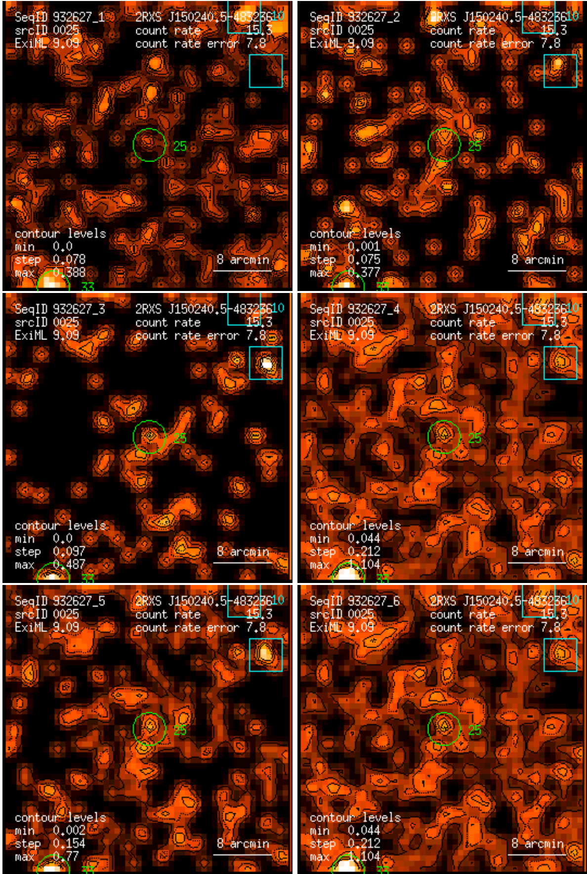
Figure 25: RASS 932627: detection 0025: band rate images, Gaussian filter: (1) PSPC channels 11 – 41, (2) 52 – 90, (3) 91 – 201, (4) 11 – 235, (5) 52 – 201, (6) 11 – 201. Broad band rates in counts/ks. Band rate contour levels in counts/ks/arcmin 2 .
