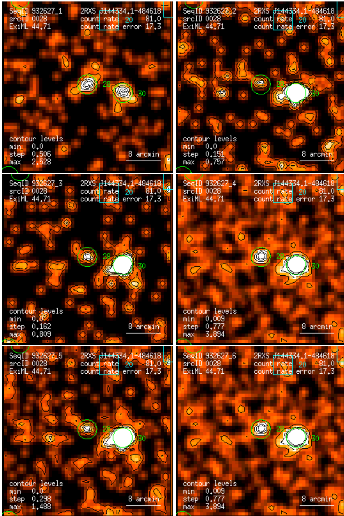
Figure 28: RASS 932627: detection 0028: band rate images, Gaussian filter: (1) PSPC channels 11 – 41, (2) 52 – 90, (3) 91 – 201, (4) 11 – 235, (5) 52 – 201, (6) 11 – 201. Broad band rates in counts/ks. Band rate contour levels in counts/ks/arcmin 2 .
