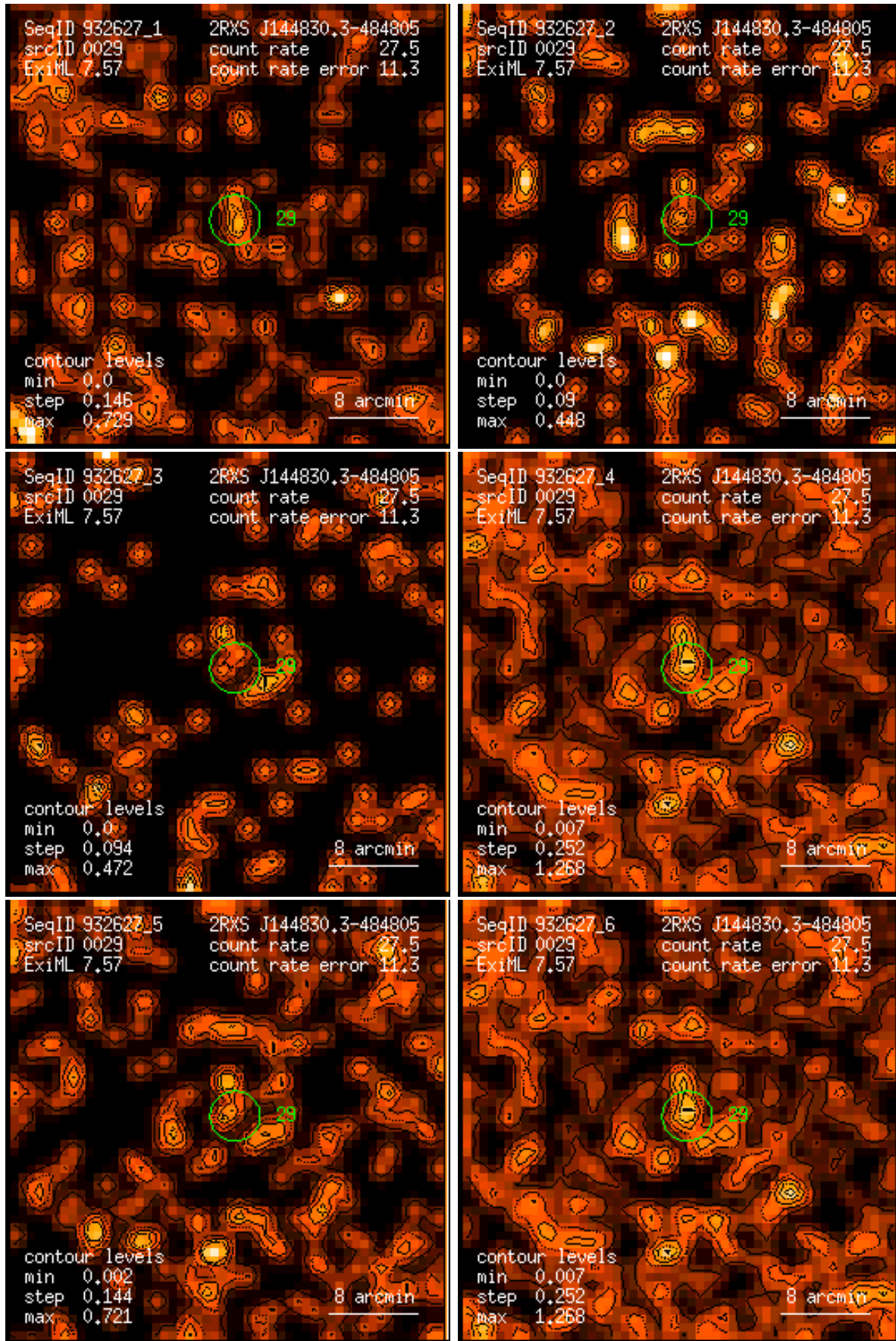
Figure 29: RASS 932627: detection 0029: band rate images, Gaussian filter: (1) PSPC channels 11 – 41, (2) 52 – 90, (3) 91 – 201, (4) 11 – 235, (5) 52 – 201, (6) 11 – 201. Broad band rates in counts/ks. Band rate contour levels in counts/ks/arcmin 2 .
