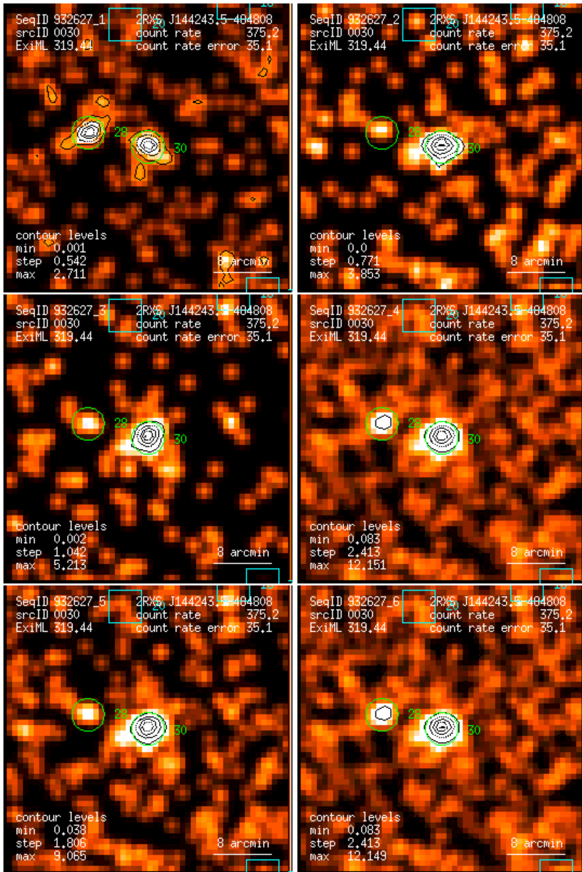
Figure 30: RASS 932627: detection 0030: band rate images, Gaussian filter: (1) PSPC channels 11 – 41, (2) 52 – 90, (3) 91 – 201, (4) 11 – 235, (5) 52 – 201, (6) 11 – 201. Broad band rates in counts/ks. Band rate contour levels in counts/ks/arcmin 2 .
