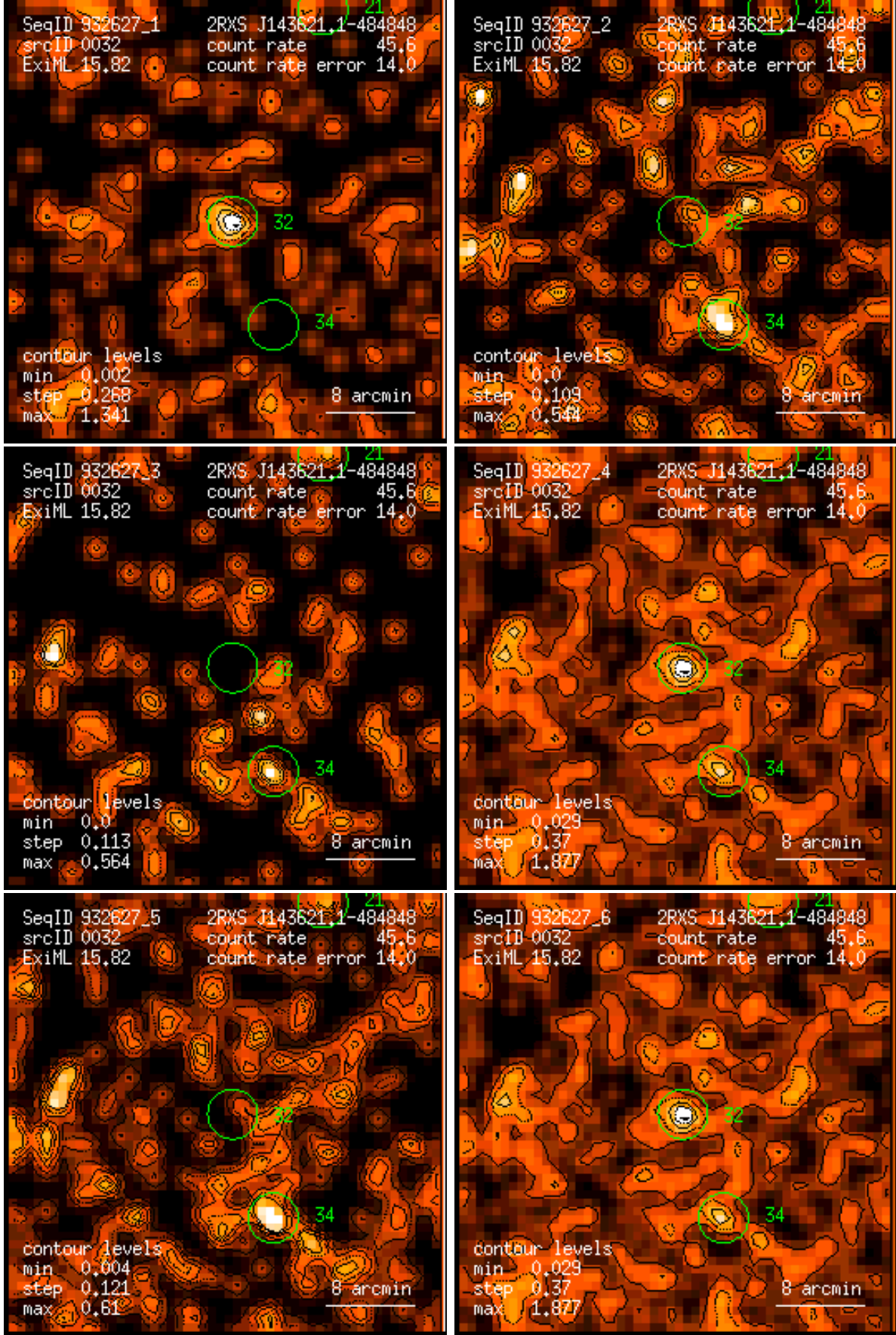
Figure 32: RASS 932627: detection 0032: band rate images, Gaussian filter: (1) PSPC channels 11 – 41, (2) 52 – 90, (3) 91 – 201, (4) 11 – 235, (5) 52 – 201, (6) 11 – 201. Broad band rates in counts/ks. Band rate contour levels in counts/ks/arcmin 2 .
