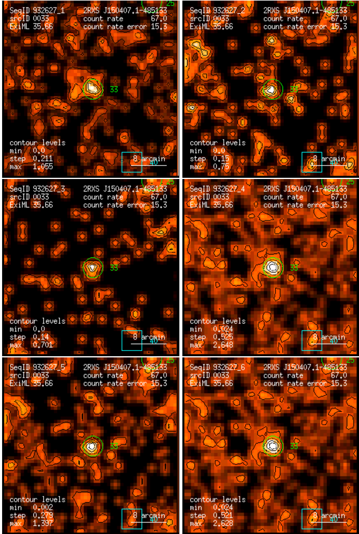
Figure 33: RASS 932627: detection 0033: band rate images, Gaussian filter: (1) PSPC channels 11 – 41, (2) 52 – 90, (3) 91 – 201, (4) 11 – 235, (5) 52 – 201, (6) 11 – 201. Broad band rates in counts/ks. Band rate contour levels in counts/ks/arcmin 2 .
