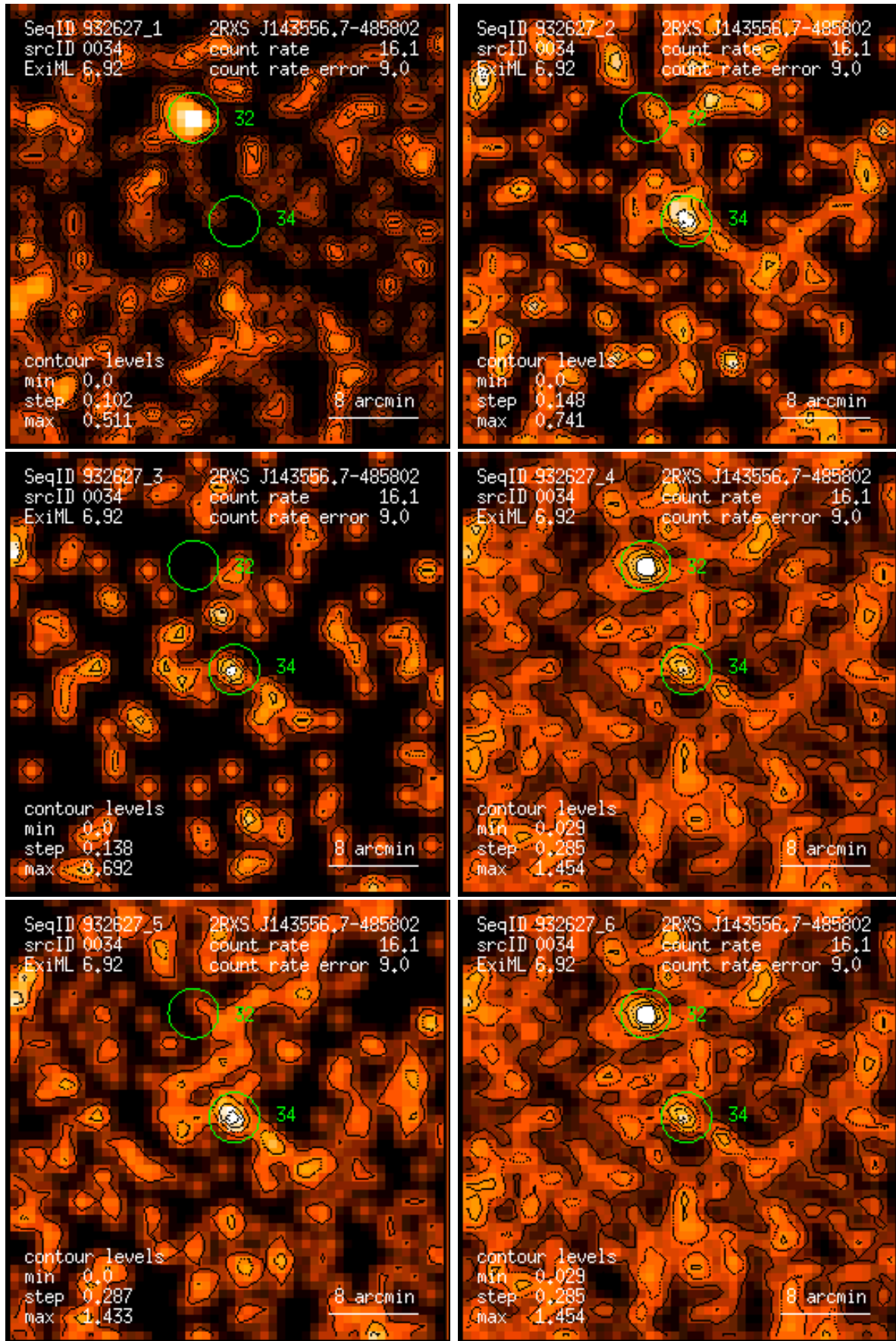
Figure 34: RASS 932627: detection 0034: band rate images, Gaussian filter: (1) PSPC channels 11 – 41, (2) 52 – 90, (3) 91 – 201, (4) 11 – 235, (5) 52 – 201, (6) 11 – 201. Broad band rates in counts/ks. Band rate contour levels in counts/ks/arcmin 2 .
