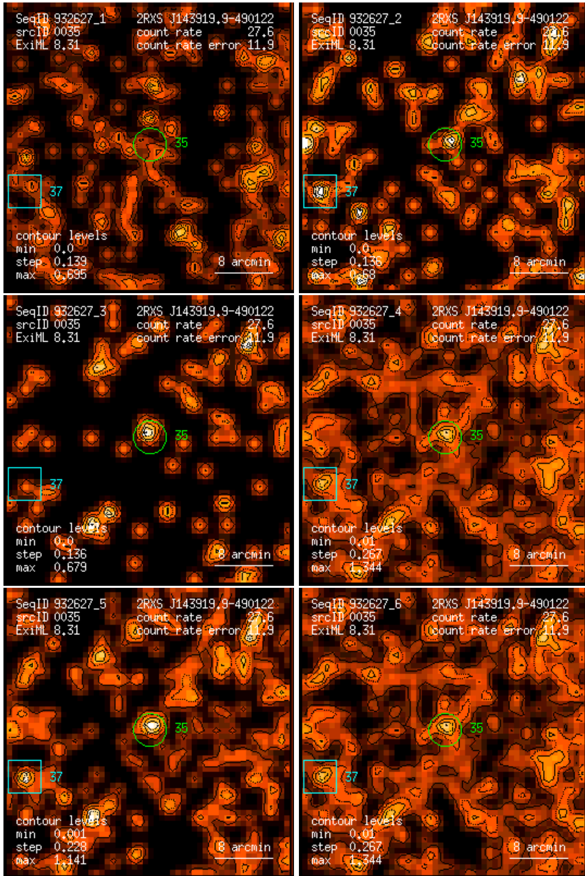
Figure 35: RASS 932627: detection 0035: band rate images, Gaussian filter: (1) PSPC channels 11 – 41, (2) 52 – 90, (3) 91 – 201, (4) 11 – 235, (5) 52 – 201, (6) 11 – 201. Broad band rates in counts/ks. Band rate contour levels in counts/ks/arcmin 2 .
