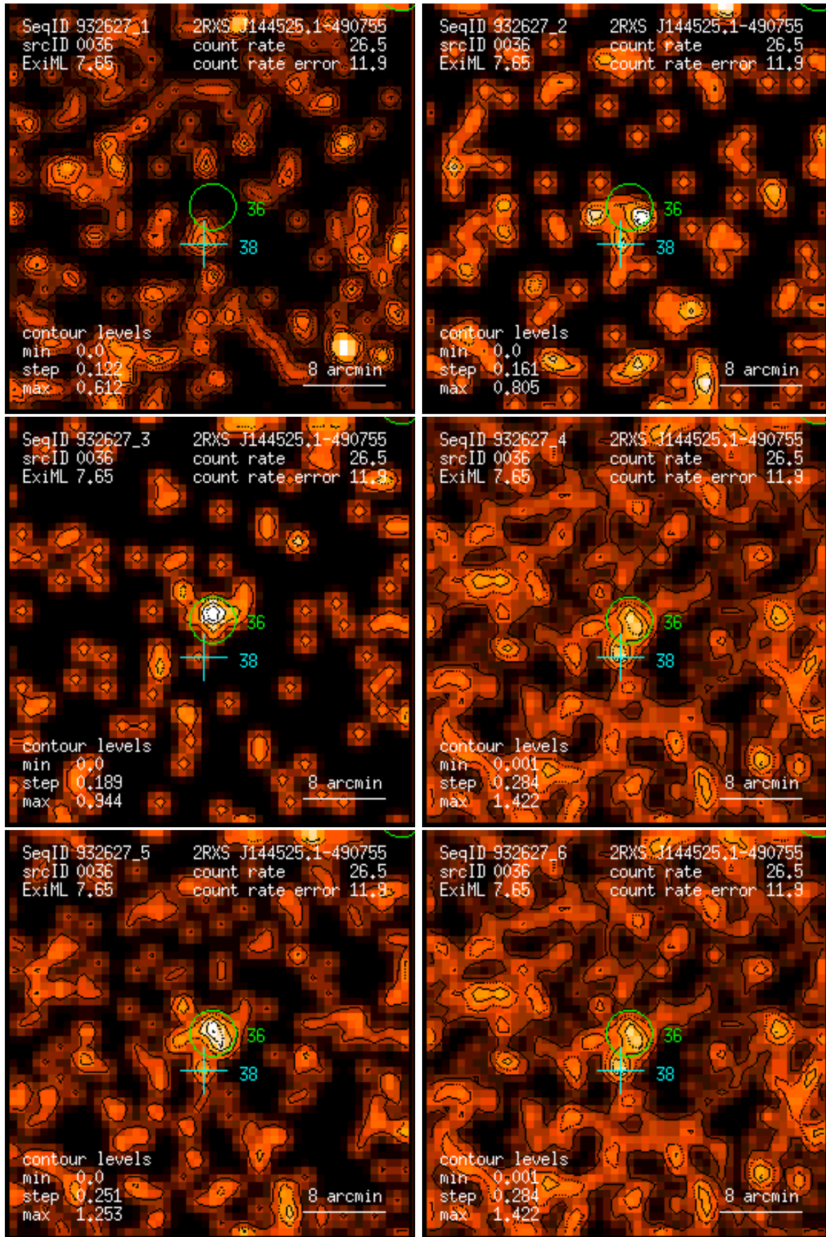
Figure 36: RASS 932627: detection 0036: band rate images, Gaussian filter: (1) PSPC channels 11 – 41, (2) 52 – 90, (3) 91 – 201, (4) 11 – 235, (5) 52 – 201, (6) 11 – 201. Broad band rates in counts/ks. Band rate contour levels in counts/ks/arcmin 2 .
