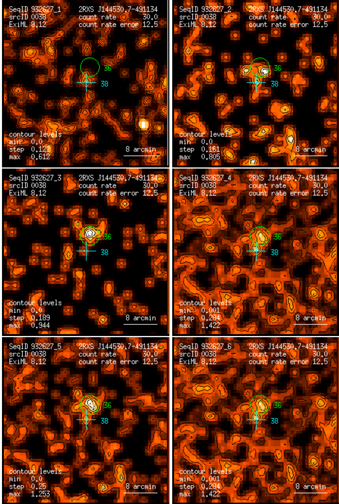
Figure 38: RASS 932627: detection 0038: band rate images, Gaussian filter: (1) PSPC channels 11 – 41, (2) 52 – 90, (3) 91 – 201, (4) 11 – 235, (5) 52 – 201, (6) 11 – 201. Broad band rates in counts/ks. Band rate contour levels in counts/ks/arcmin 2 .
