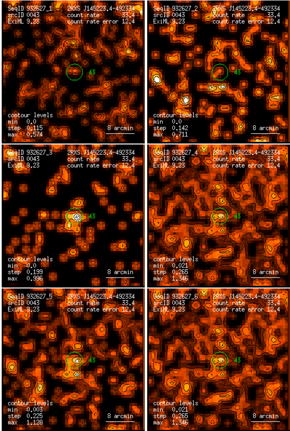
Figure 43: RASS 932627: detection 0043: band rate images, Gaussian filter: (1) PSPC channels 11 – 41, (2) 52 – 90, (3) 91 – 201, (4) 11 – 235, (5) 52 – 201, (6) 11 – 201. Broad band rates in counts/ks. Band rate contour levels in counts/ks/arcmin 2 .
