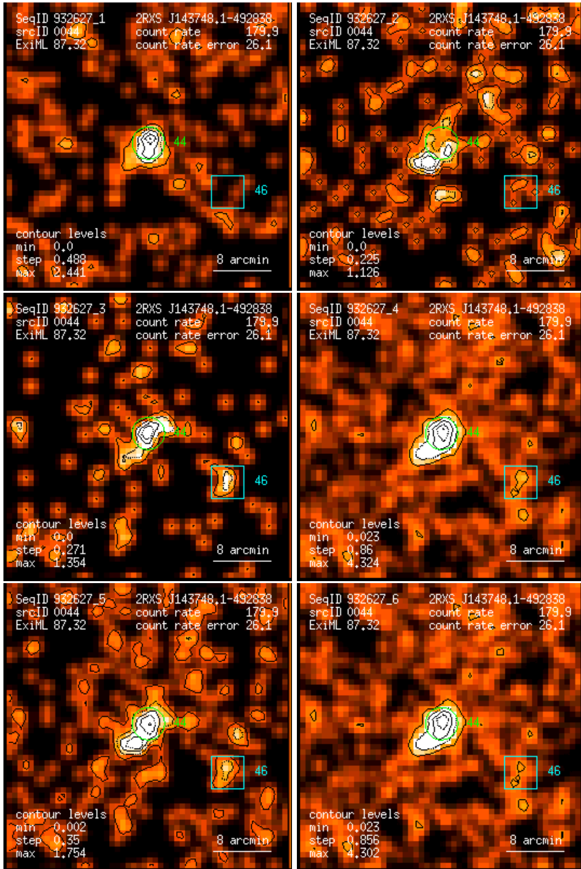
Figure 44: RASS 932627: detection 0044: band rate images, Gaussian filter: (1) PSPC channels 11 – 41, (2) 52 – 90, (3) 91 – 201, (4) 11 – 235, (5) 52 – 201, (6) 11 – 201. Broad band rates in counts/ks. Band rate contour levels in counts/ks/arcmin 2 .
