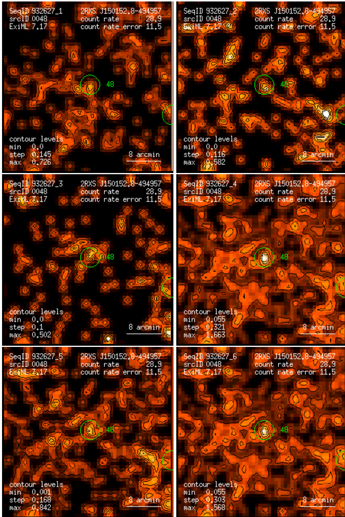
Figure 48: RASS 932627: detection 0048: band rate images, Gaussian filter: (1) PSPC channels 11 – 41, (2) 52 – 90, (3) 91 – 201, (4) 11 – 235, (5) 52 – 201, (6) 11 – 201. Broad band rates in counts/ks. Band rate contour levels in counts/ks/arcmin 2 .
