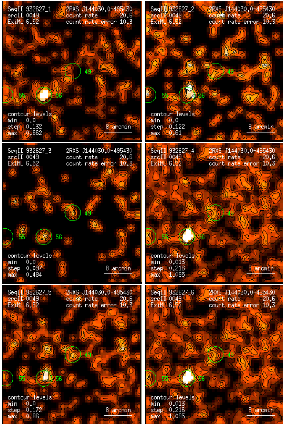
Figure 49: RASS 932627: detection 0049: band rate images, Gaussian filter: (1) PSPC channels 11 – 41, (2) 52 – 90, (3) 91 – 201, (4) 11 – 235, (5) 52 – 201, (6) 11 – 201. Broad band rates in counts/ks. Band rate contour levels in counts/ks/arcmin 2 .
