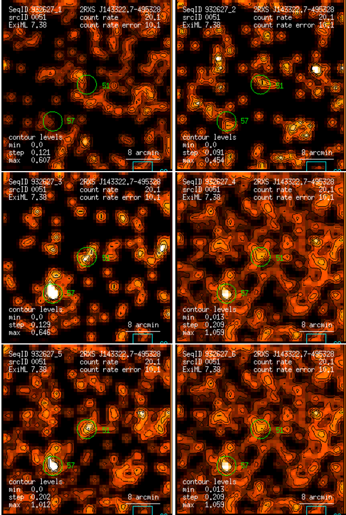
Figure 51: RASS 932627: detection 0051: band rate images, Gaussian filter: (1) PSPC channels 11 – 41, (2) 52 – 90, (3) 91 – 201, (4) 11 – 235, (5) 52 – 201, (6) 11 – 201. Broad band rates in counts/ks. Band rate contour levels in counts/ks/arcmin 2 .
