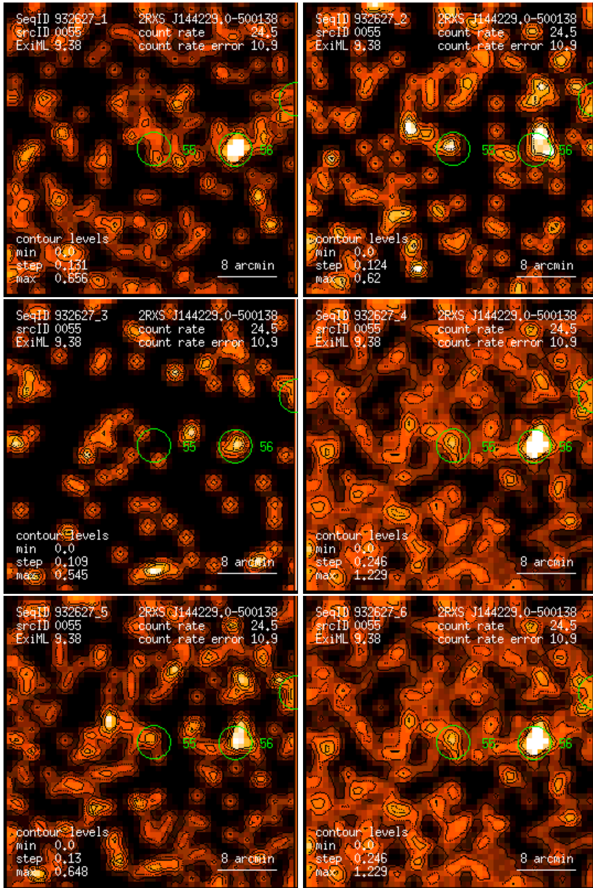
Figure 55: RASS 932627: detection 0055: band rate images, Gaussian filter: (1) PSPC channels 11 – 41, (2) 52 – 90, (3) 91 – 201, (4) 11 – 235, (5) 52 – 201, (6) 11 – 201. Broad band rates in counts/ks. Band rate contour levels in counts/ks/arcmin 2 .
