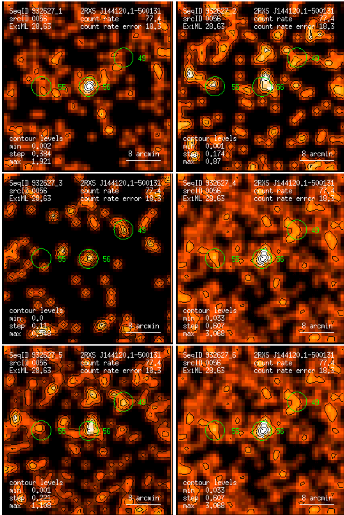
Figure 56: RASS 932627: detection 0056: band rate images, Gaussian filter: (1) PSPC channels 11 – 41, (2) 52 – 90, (3) 91 – 201, (4) 11 – 235, (5) 52 – 201, (6) 11 – 201. Broad band rates in counts/ks. Band rate contour levels in counts/ks/arcmin 2 .
