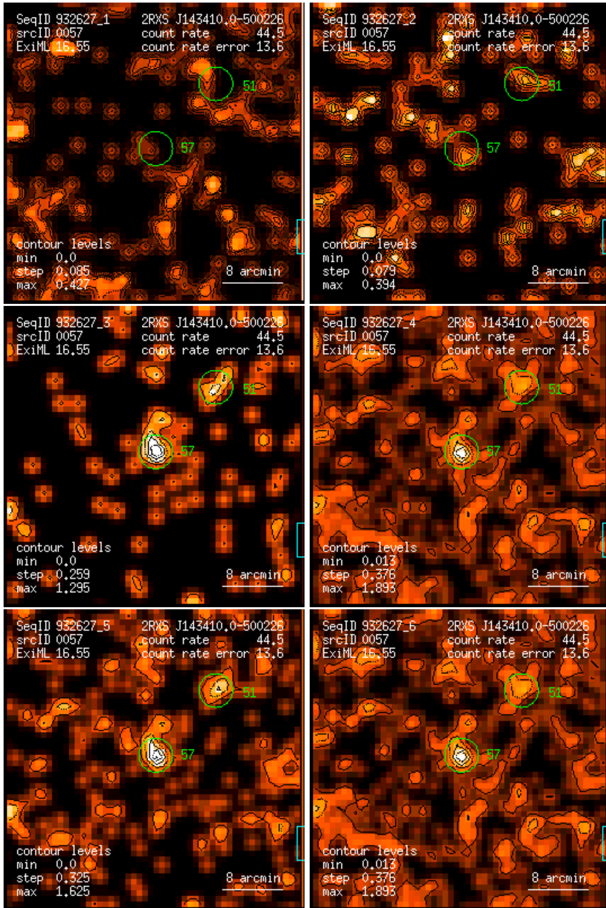
Figure 57: RASS 932627: detection 0057: band rate images, Gaussian filter: (1) PSPC channels 11 – 41, (2) 52 – 90, (3) 91 – 201, (4) 11 – 235, (5) 52 – 201, (6) 11 – 201. Broad band rates in counts/ks. Band rate contour levels in counts/ks/arcmin 2 .
