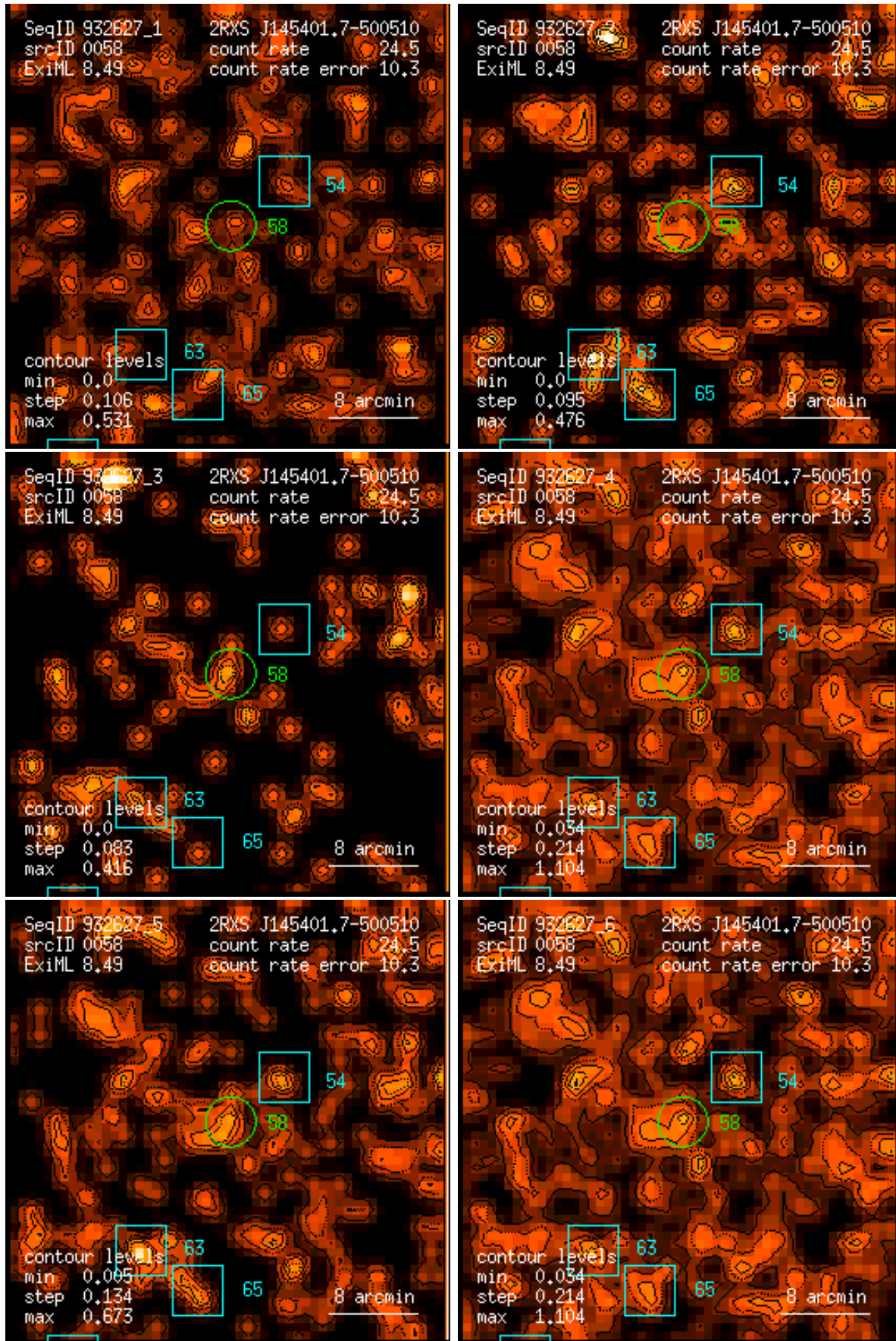
Figure 58: RASS 932627: detection 0058: band rate images, Gaussian filter: (1) PSPC channels 11 – 41, (2) 52 – 90, (3) 91 – 201, (4) 11 – 235, (5) 52 – 201, (6) 11 – 201. Broad band rates in counts/ks. Band rate contour levels in counts/ks/arcmin 2 .
