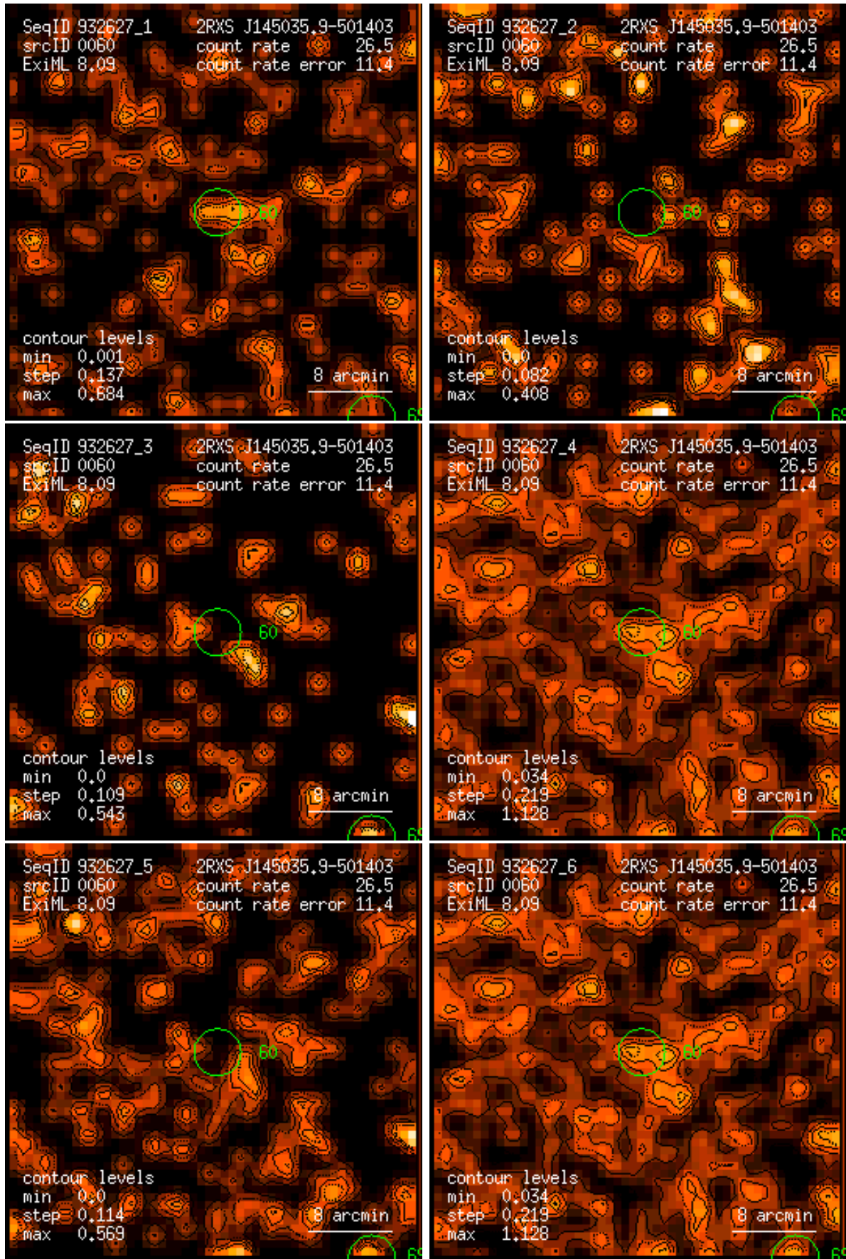
Figure 60: RASS 932627: detection 0060: band rate images, Gaussian filter: (1) PSPC channels 11 – 41, (2) 52 – 90, (3) 91 – 201, (4) 11 – 235, (5) 52 – 201, (6) 11 – 201. Broad band rates in counts/ks. Band rate contour levels in counts/ks/arcmin 2 .
