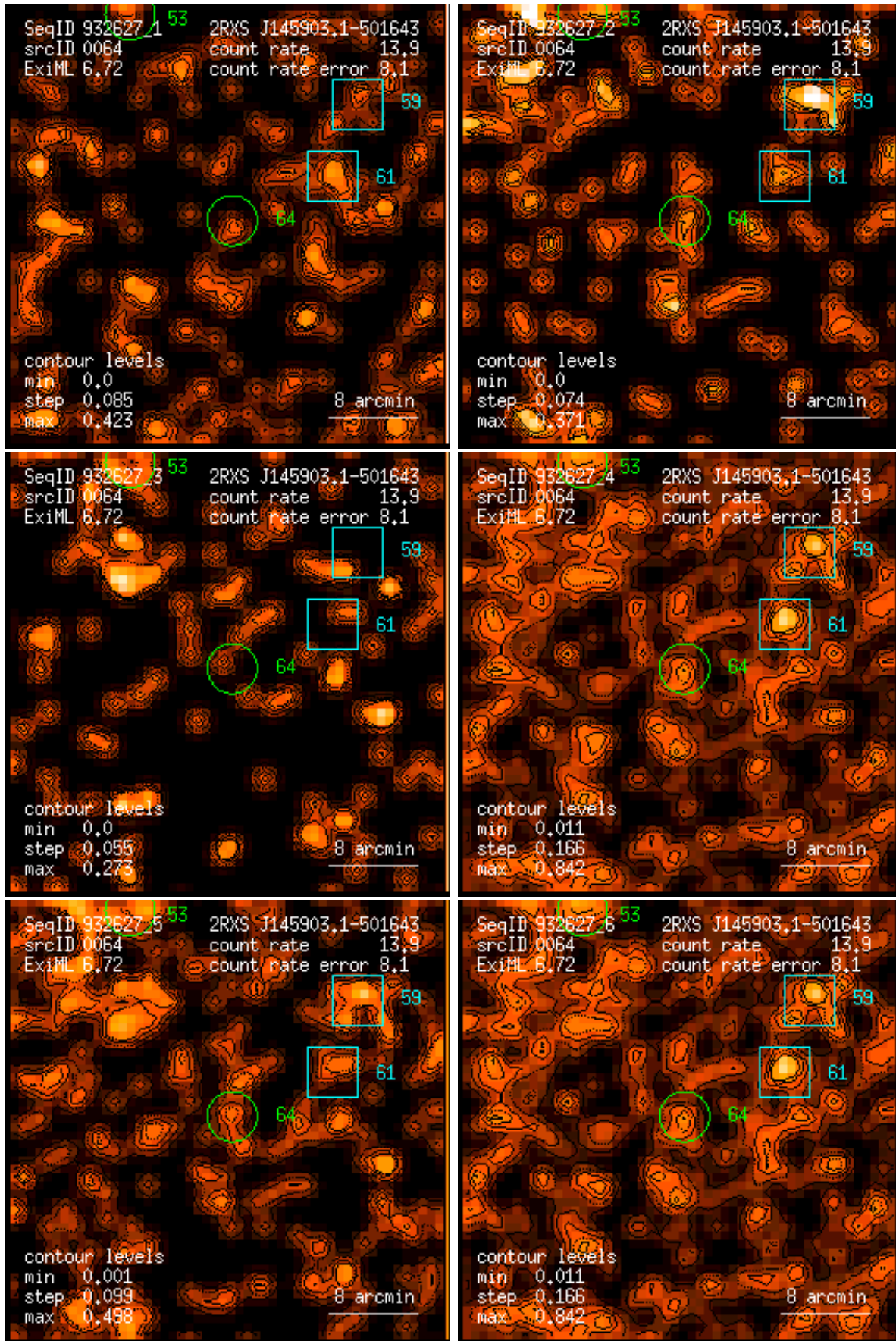
Figure 64: RASS 932627: detection 0064: band rate images, Gaussian filter: (1) PSPC channels 11 – 41, (2) 52 – 90, (3) 91 – 201, (4) 11 – 235, (5) 52 – 201, (6) 11 – 201. Broad band rates in counts/ks. Band rate contour levels in counts/ks/arcmin 2 .
