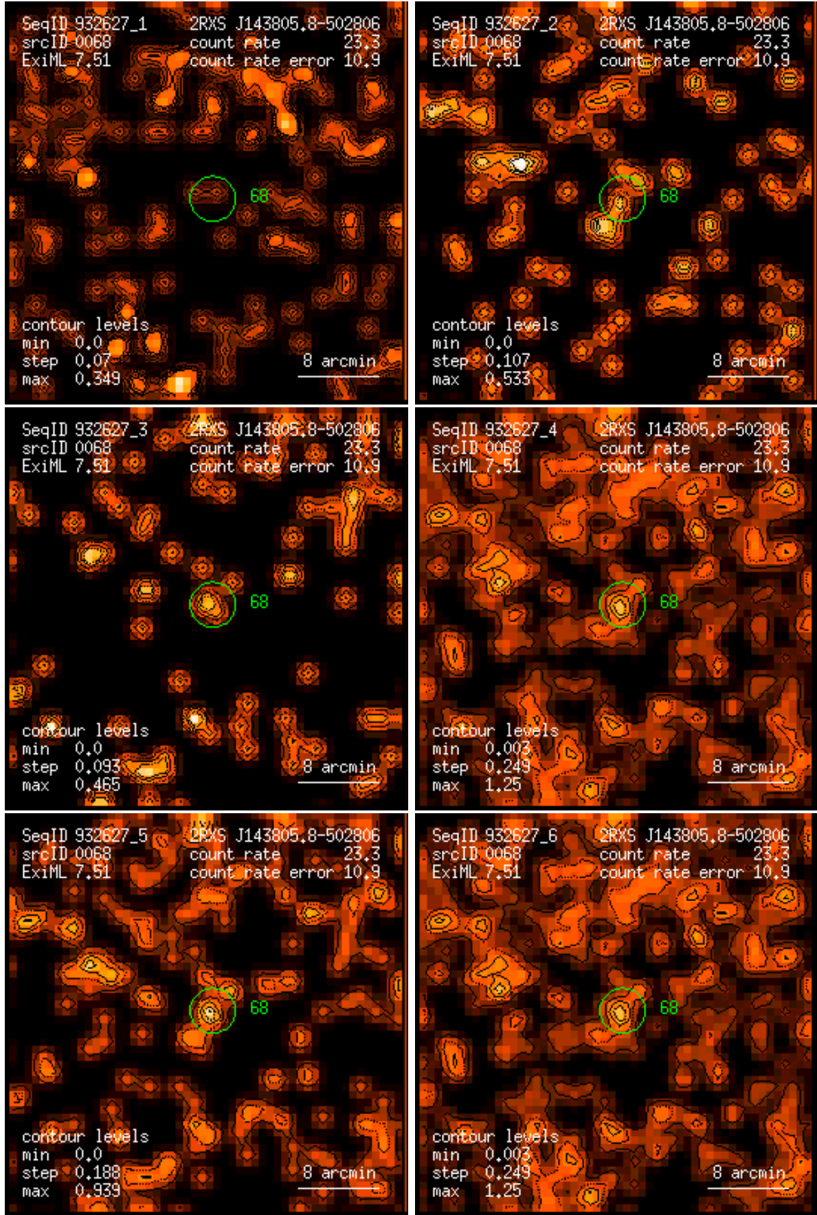
Figure 68: RASS 932627: detection 0068: band rate images, Gaussian filter: (1) PSPC channels 11 – 41, (2) 52 – 90, (3) 91 – 201, (4) 11 – 235, (5) 52 – 201, (6) 11 – 201. Broad band rates in counts/ks. Band rate contour levels in counts/ks/arcmin 2 .
