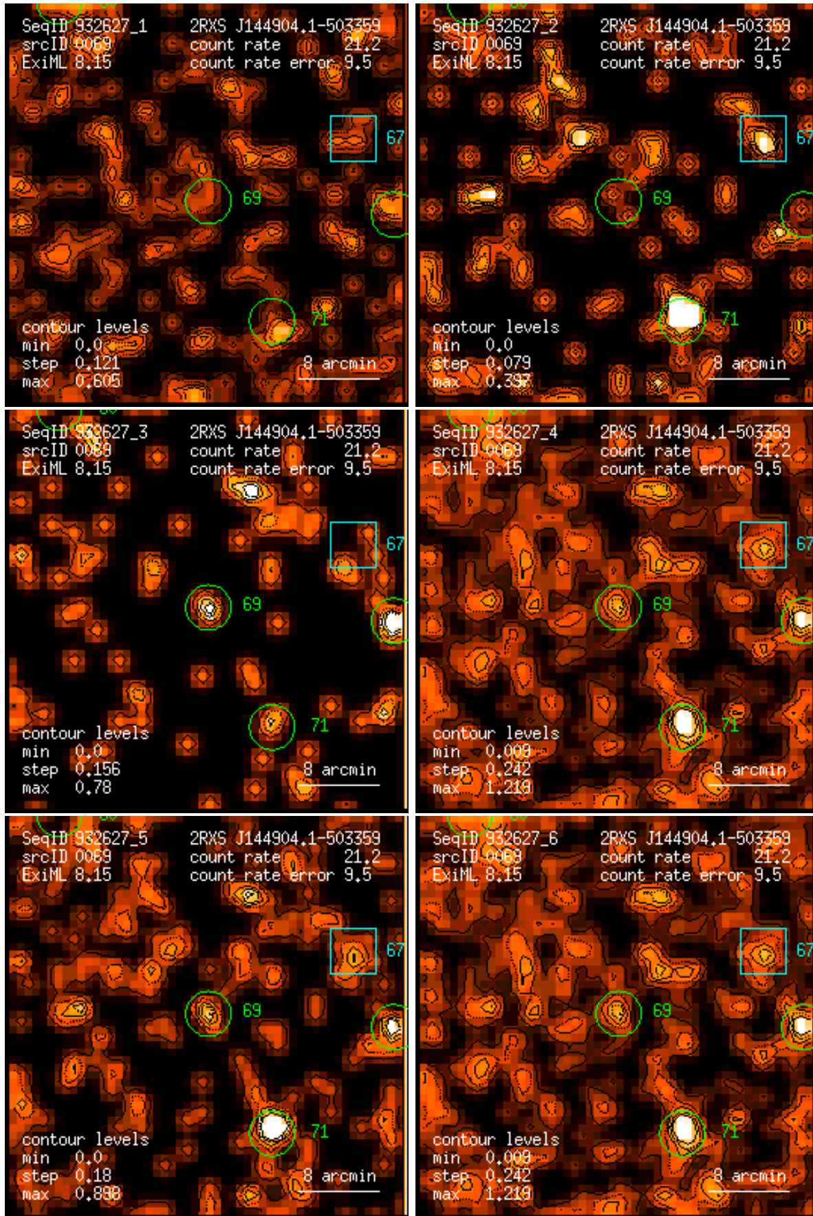
Figure 69: RASS 932627: detection 0069: band rate images, Gaussian filter: (1) PSPC channels 11 – 41, (2) 52 – 90, (3) 91 – 201, (4) 11 – 235, (5) 52 – 201, (6) 11 – 201. Broad band rates in counts/ks. Band rate contour levels in counts/ks/arcmin 2 .
