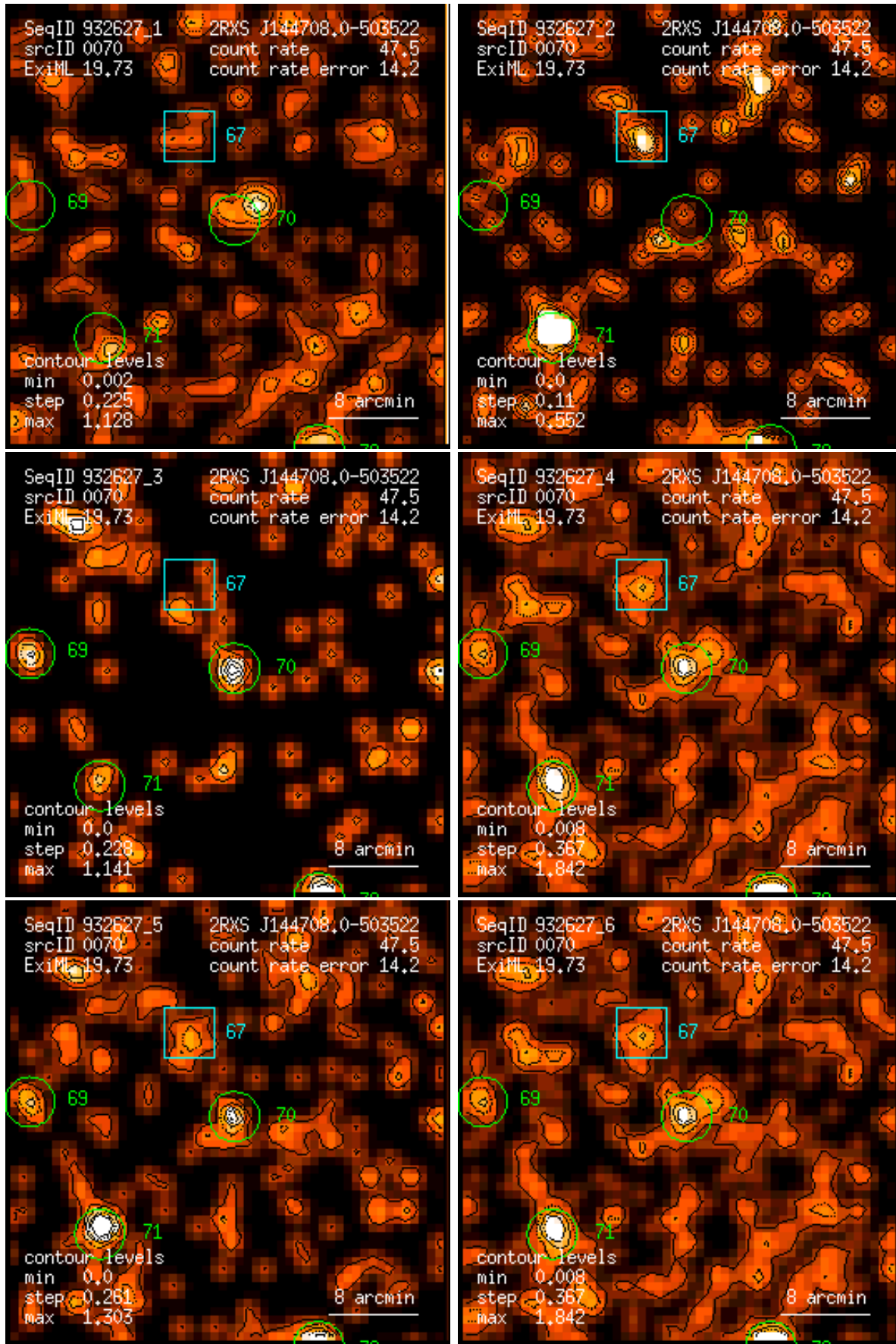
Figure 70: RASS 932627: detection 0070: band rate images, Gaussian filter: (1) PSPC channels 11 – 41, (2) 52 – 90, (3) 91 – 201, (4) 11 – 235, (5) 52 – 201, (6) 11 – 201. Broad band rates in counts/ks. Band rate contour levels in counts/ks/arcmin 2 .
