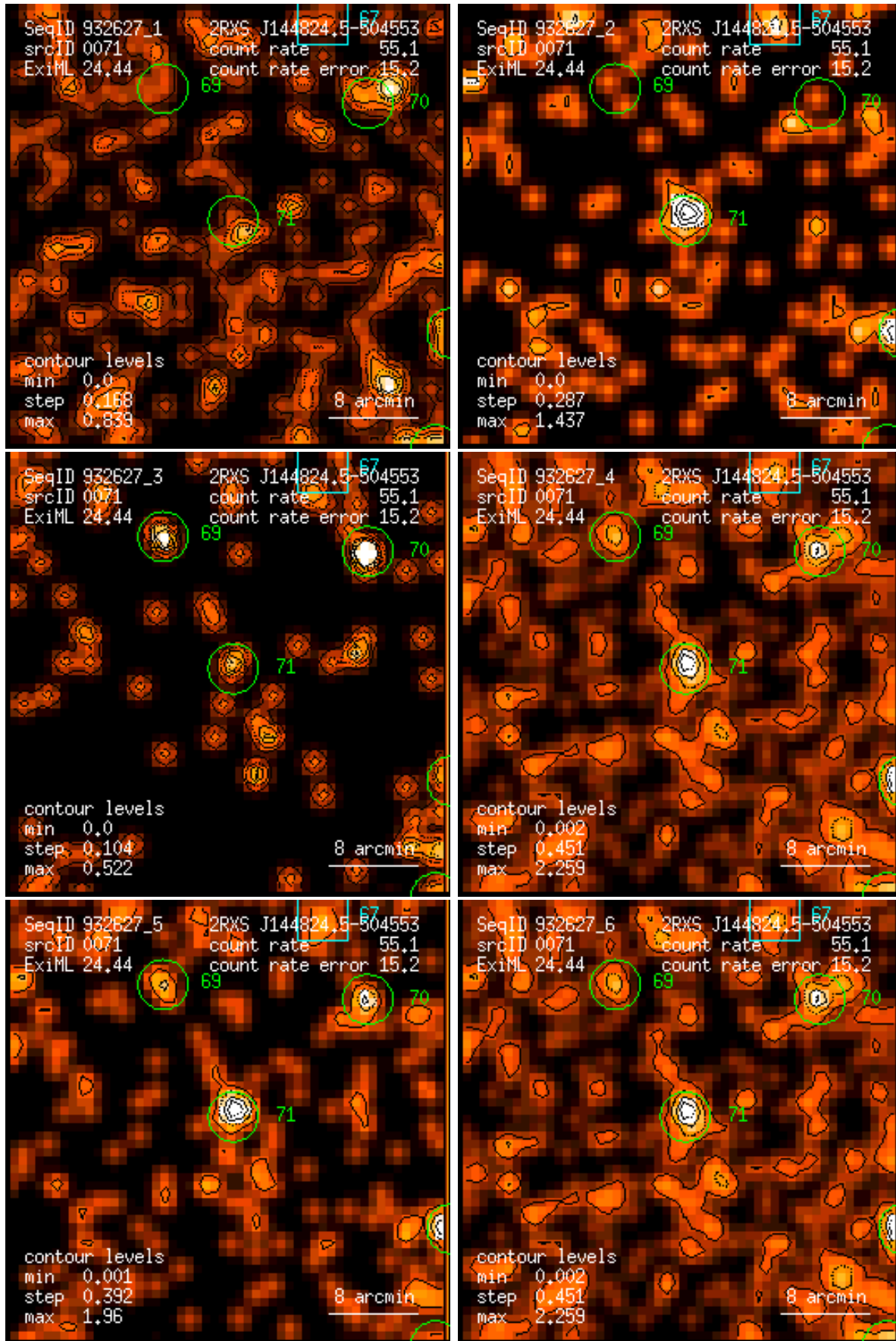
Figure 71: RASS 932627: detection 0071: band rate images, Gaussian filter: (1) PSPC channels 11 – 41, (2) 52 – 90, (3) 91 – 201, (4) 11 – 235, (5) 52 – 201, (6) 11 – 201. Broad band rates in counts/ks. Band rate contour levels in counts/ks/arcmin 2 .
