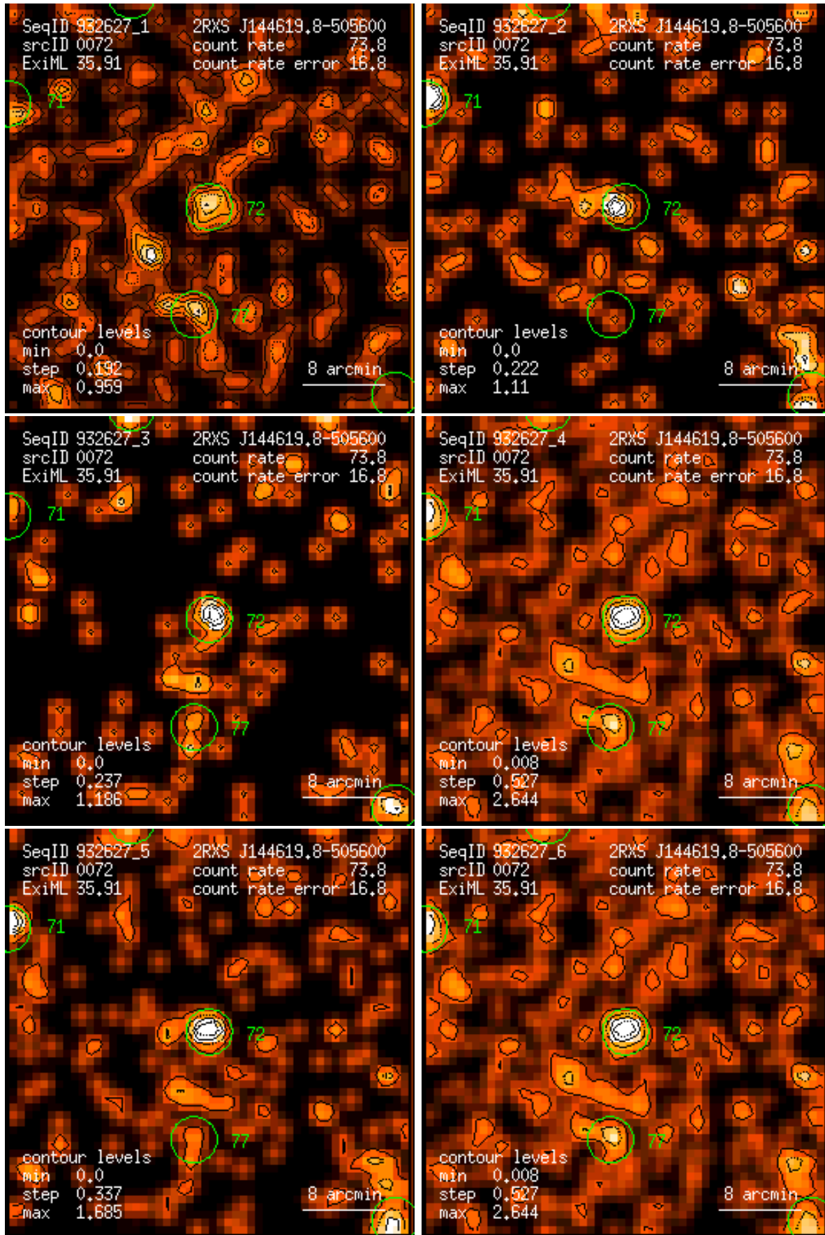
Figure 72: RASS 932627: detection 0072: band rate images, Gaussian filter: (1) PSPC channels 11 – 41, (2) 52 – 90, (3) 91 – 201, (4) 11 – 235, (5) 52 – 201, (6) 11 – 201. Broad band rates in counts/ks. Band rate contour levels in counts/ks/arcmin 2 .
