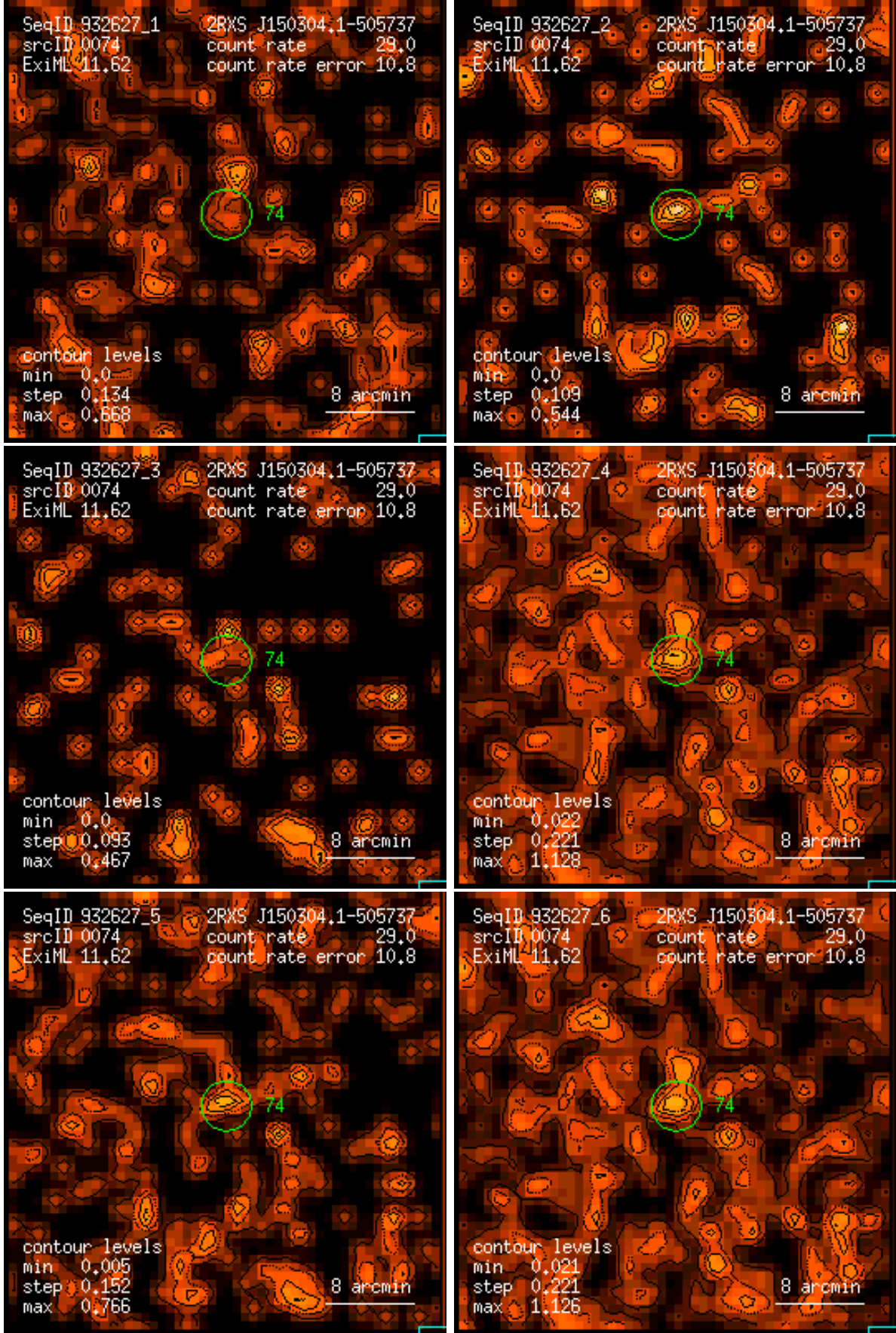
Figure 74: RASS 932627: detection 0074: band rate images, Gaussian filter: (1) PSPC channels 11 – 41, (2) 52 – 90, (3) 91 – 201, (4) 11 – 235, (5) 52 – 201, (6) 11 – 201. Broad band rates in counts/ks. Band rate contour levels in counts/ks/arcmin 2 .
