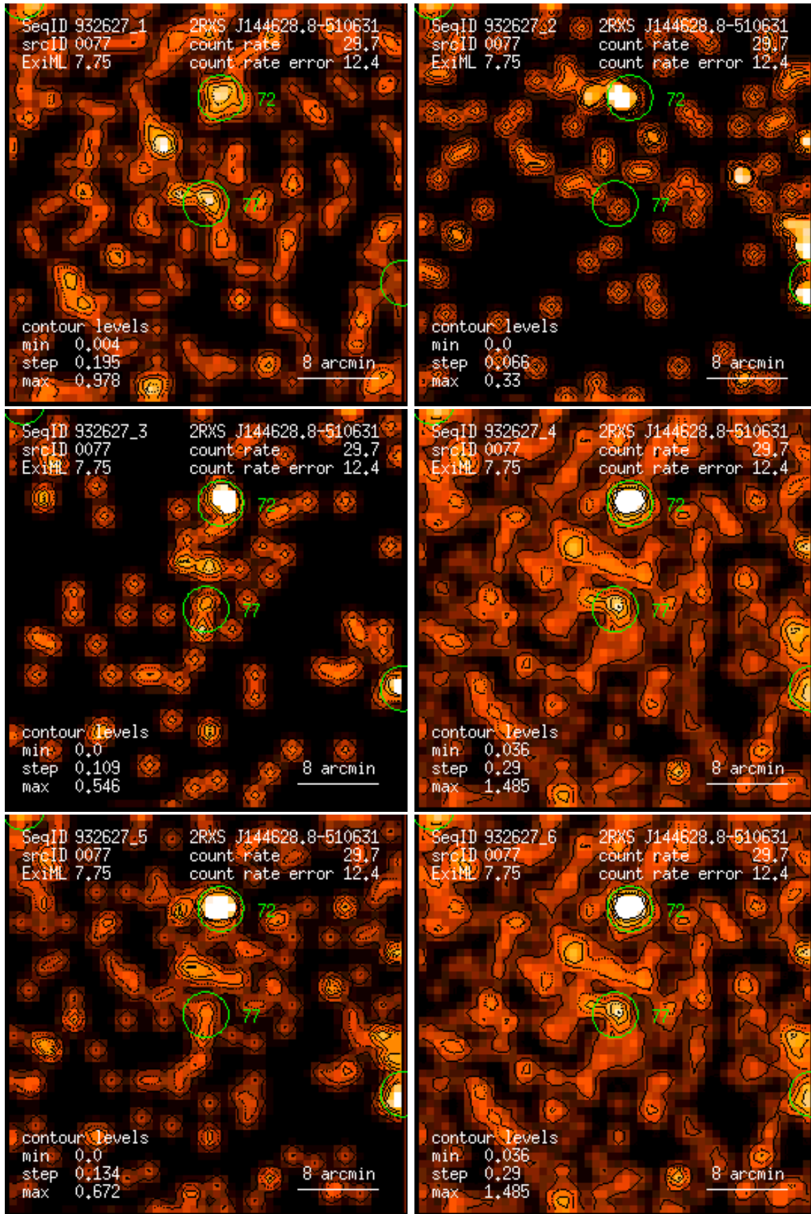
Figure 77: RASS 932627: detection 0077: band rate images, Gaussian filter: (1) PSPC channels 11 – 41, (2) 52 – 90, (3) 91 – 201, (4) 11 – 235, (5) 52 – 201, (6) 11 – 201. Broad band rates in counts/ks. Band rate contour levels in counts/ks/arcmin 2 .
