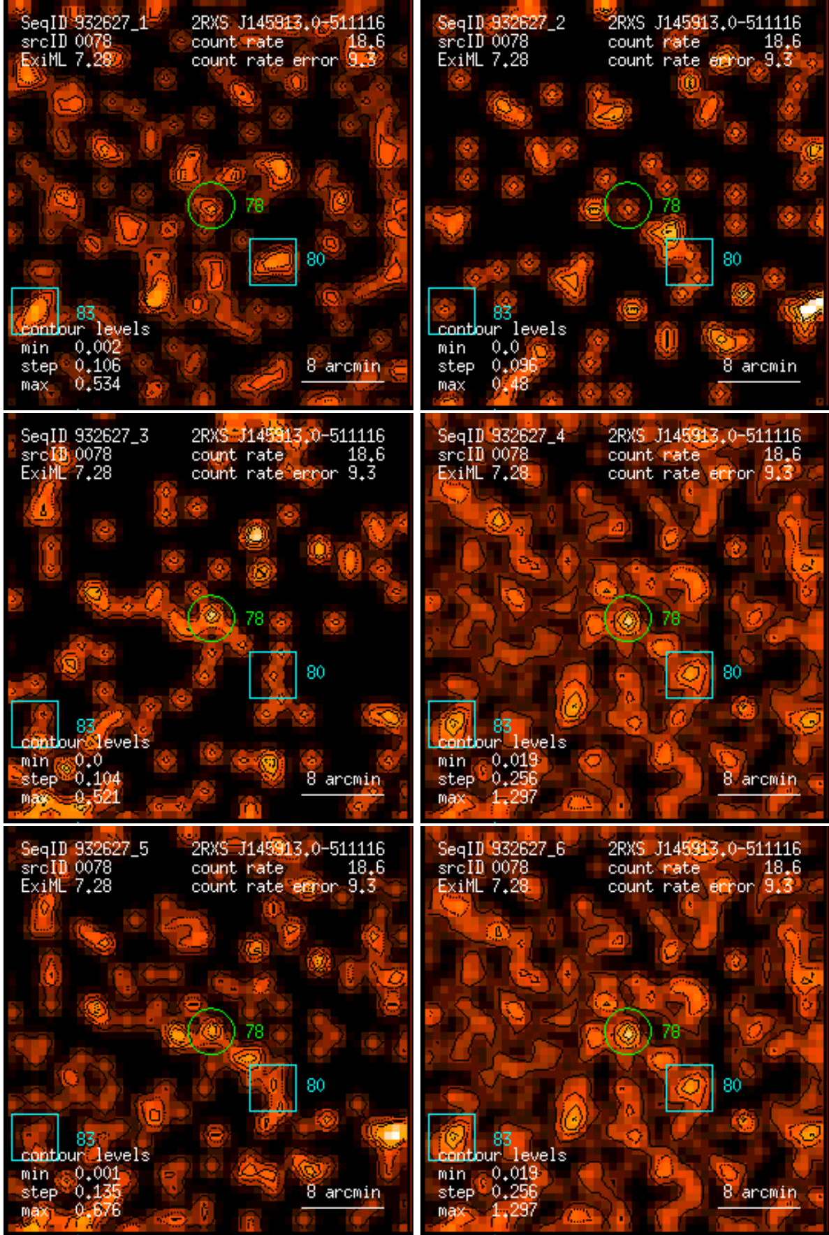
Figure 78: RASS 932627: detection 0078: band rate images, Gaussian filter: (1) PSPC channels 11 – 41, (2) 52 – 90, (3) 91 – 201, (4) 11 – 235, (5) 52 – 201, (6) 11 – 201. Broad band rates in counts/ks. Band rate contour levels in counts/ks/arcmin 2 .
