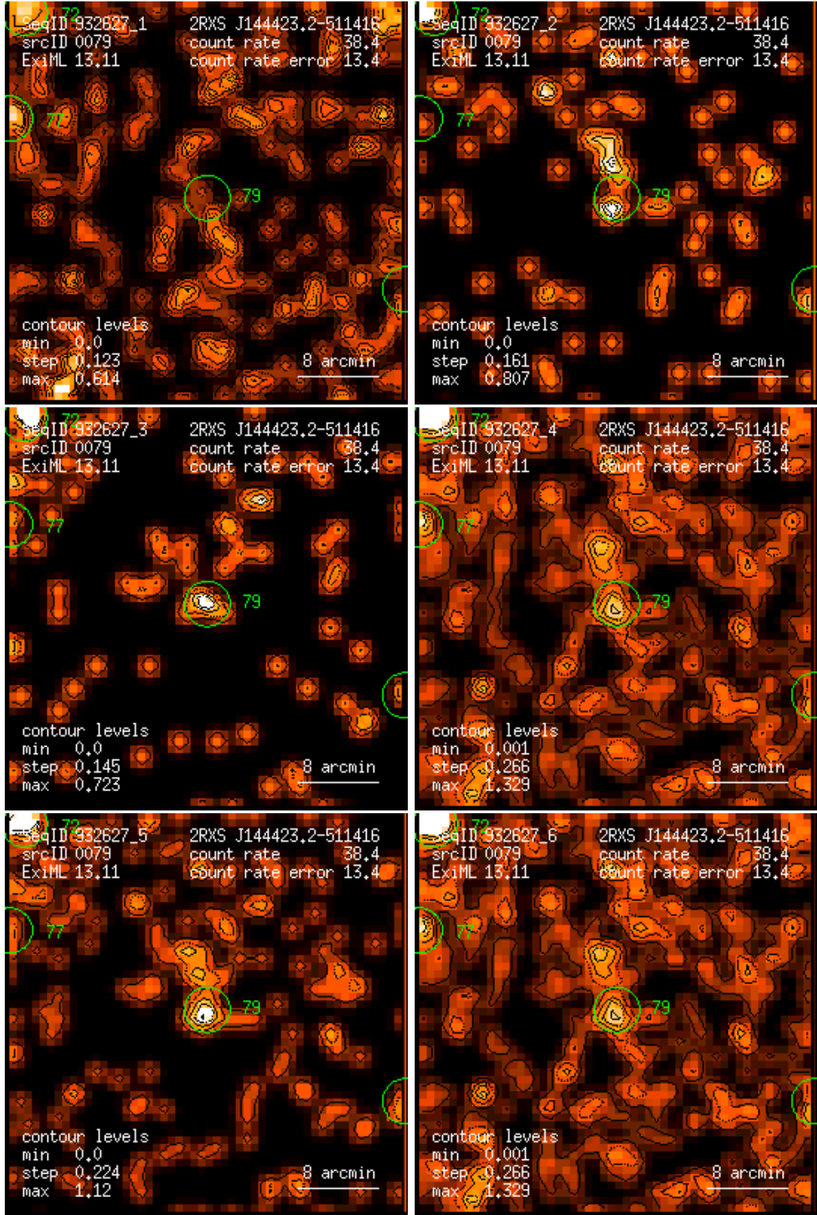
Figure 79: RASS 932627: detection 0079: band rate images, Gaussian filter: (1) PSPC channels 11 – 41, (2) 52 – 90, (3) 91 – 201, (4) 11 – 235, (5) 52 – 201, (6) 11 – 201. Broad band rates in counts/ks. Band rate contour levels in counts/ks/arcmin 2 .
