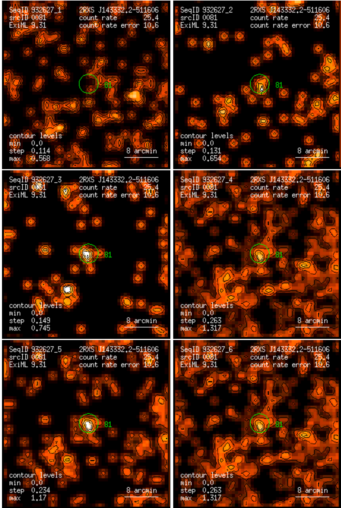
Figure 81: RASS 932627: detection 0081: band rate images, Gaussian filter: (1) PSPC channels 11 – 41, (2) 52 – 90, (3) 91 – 201, (4) 11 – 235, (5) 52 – 201, (6) 11 – 201. Broad band rates in counts/ks. Band rate contour levels in counts/ks/arcmin 2 .
