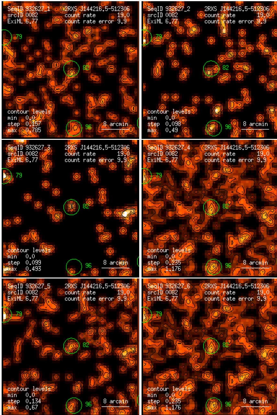
Figure 82: RASS 932627: detection 0082: band rate images, Gaussian filter: (1) PSPC channels 11 – 41, (2) 52 – 90, (3) 91 – 201, (4) 11 – 235, (5) 52 – 201, (6) 11 – 201. Broad band rates in counts/ks. Band rate contour levels in counts/ks/arcmin 2 .
