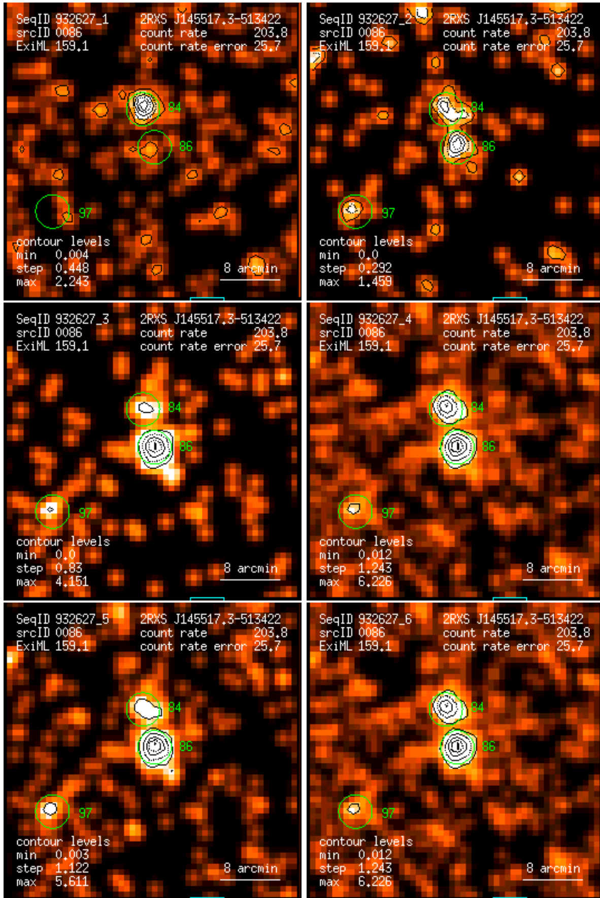
Figure 86: RASS 932627: detection 0086: band rate images, Gaussian filter: (1) PSPC channels 11 – 41, (2) 52 – 90, (3) 91 – 201, (4) 11 – 235, (5) 52 – 201, (6) 11 – 201. Broad band rates in counts/ks. Band rate contour levels in counts/ks/arcmin 2 .
