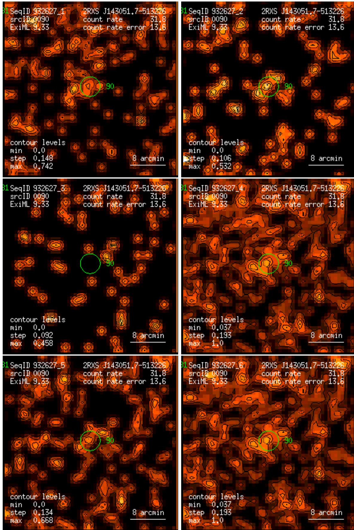
Figure 90: RASS 932627: detection 0090: band rate images, Gaussian filter: (1) PSPC channels 11 – 41, (2) 52 – 90, (3) 91 – 201, (4) 11 – 235, (5) 52 – 201, (6) 11 – 201. Broad band rates in counts/ks. Band rate contour levels in counts/ks/arcmin 2 .
