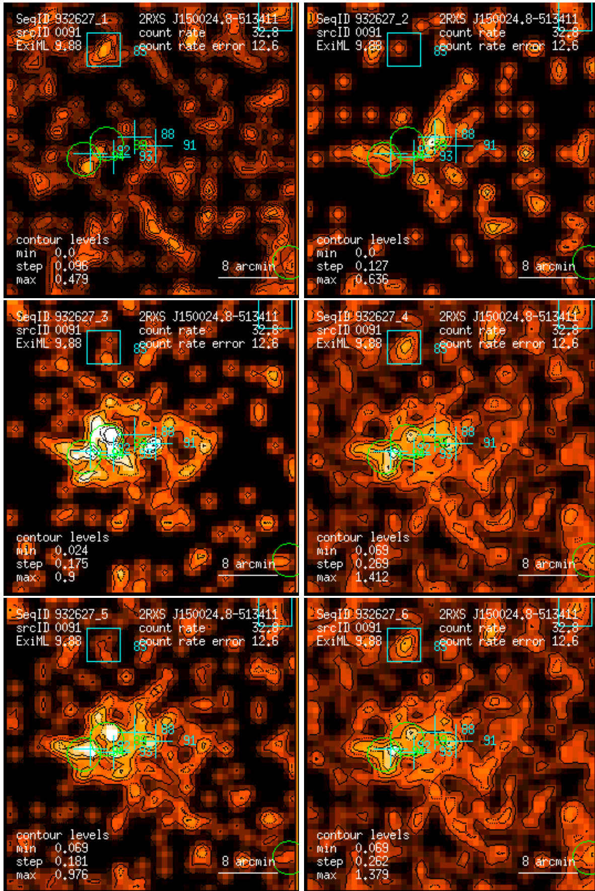
Figure 91: RASS 932627: detection 0091: band rate images, Gaussian filter: (1) PSPC channels 11 – 41, (2) 52 – 90, (3) 91 – 201, (4) 11 – 235, (5) 52 – 201, (6) 11 – 201. Broad band rates in counts/ks. Band rate contour levels in counts/ks/arcmin 2 .
