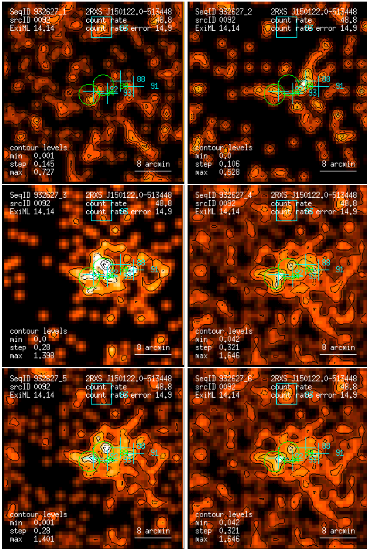
Figure 92: RASS 932627: detection 0092: band rate images, Gaussian filter: (1) PSPC channels 11 – 41, (2) 52 – 90, (3) 91 – 201, (4) 11 – 235, (5) 52 – 201, (6) 11 – 201. Broad band rates in counts/ks. Band rate contour levels in counts/ks/arcmin 2 .
