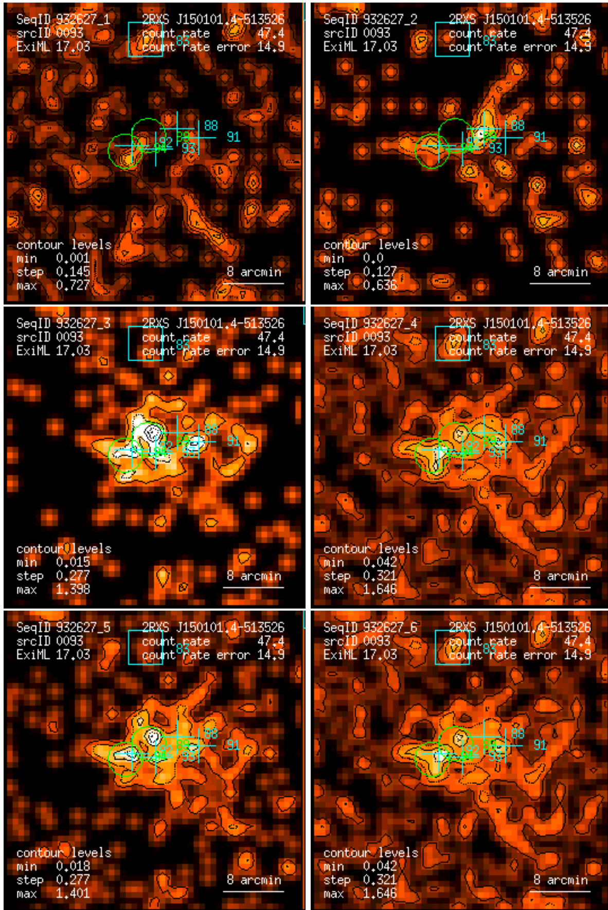
Figure 93: RASS 932627: detection 0093: band rate images, Gaussian filter: (1) PSPC channels 11 – 41, (2) 52 – 90, (3) 91 – 201, (4) 11 – 235, (5) 52 – 201, (6) 11 – 201. Broad band rates in counts/ks. Band rate contour levels in counts/ks/arcmin 2 .
