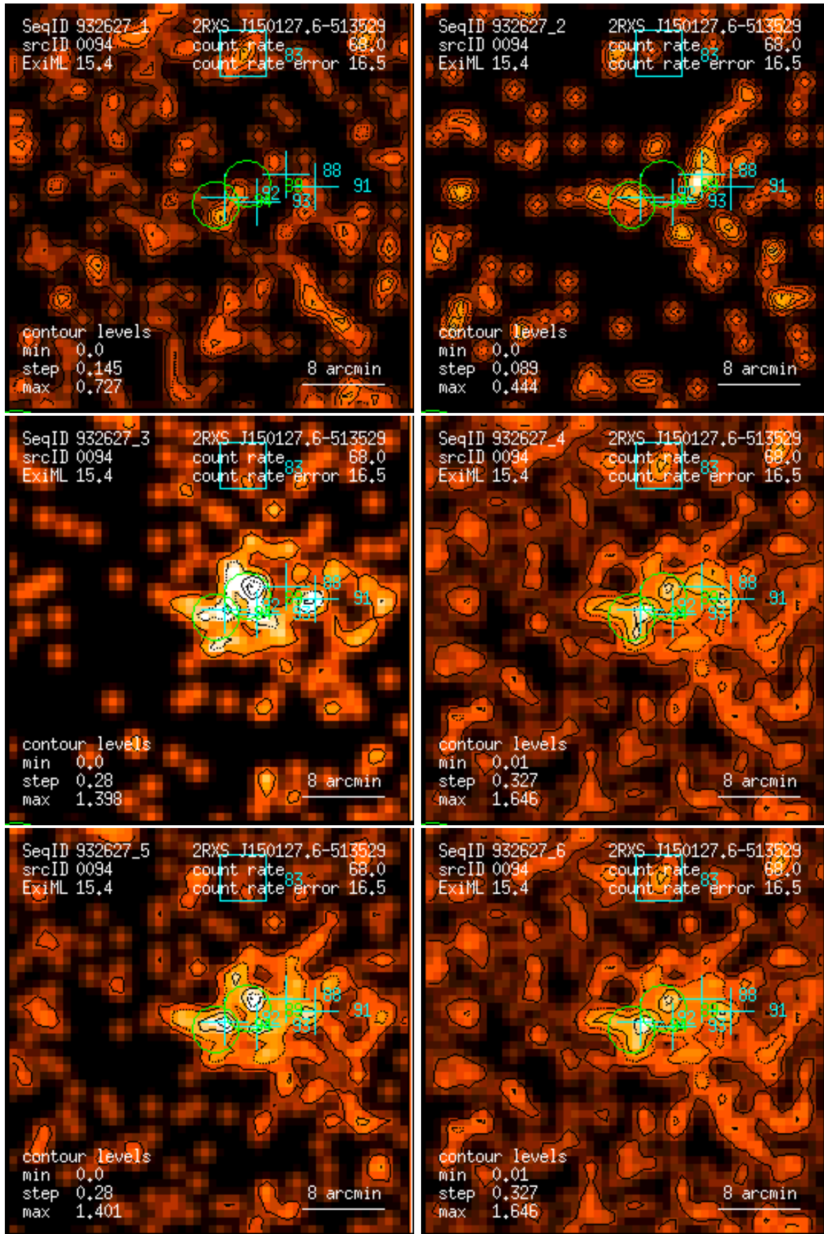
Figure 94: RASS 932627: detection 0094: band rate images, Gaussian filter: (1) PSPC channels 11 – 41, (2) 52 – 90, (3) 91 – 201, (4) 11 – 235, (5) 52 – 201, (6) 11 – 201. Broad band rates in counts/ks. Band rate contour levels in counts/ks/arcmin 2 .
