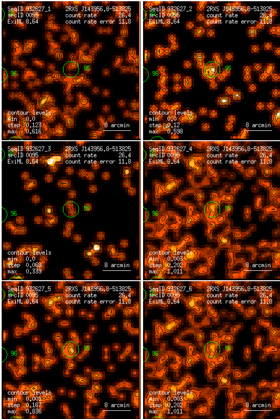
Figure 95: RASS 932627: detection 0095: band rate images, Gaussian filter: (1) PSPC channels 11 – 41, (2) 52 – 90, (3) 91 – 201, (4) 11 – 235, (5) 52 – 201, (6) 11 – 201. Broad band rates in counts/ks. Band rate contour levels in counts/ks/arcmin 2 .
