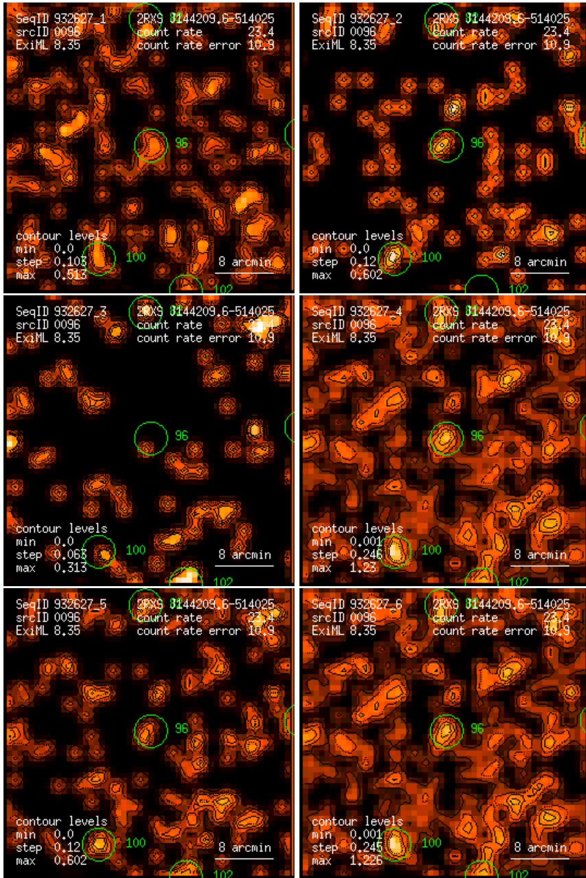
Figure 96: RASS 932627: detection 0096: band rate images, Gaussian filter: (1) PSPC channels 11 – 41, (2) 52 – 90, (3) 91 – 201, (4) 11 – 235, (5) 52 – 201, (6) 11 – 201. Broad band rates in counts/ks. Band rate contour levels in counts/ks/arcmin 2 .
