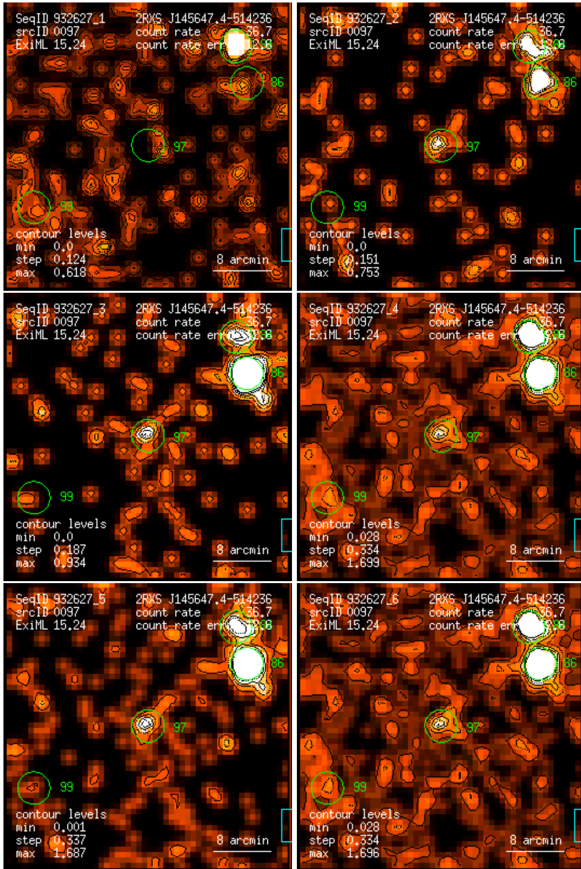
Figure 97: RASS 932627: detection 0097: band rate images, Gaussian filter: (1) PSPC channels 11 – 41, (2) 52 – 90, (3) 91 – 201, (4) 11 – 235, (5) 52 – 201, (6) 11 – 201. Broad band rates in counts/ks. Band rate contour levels in counts/ks/arcmin 2 .
