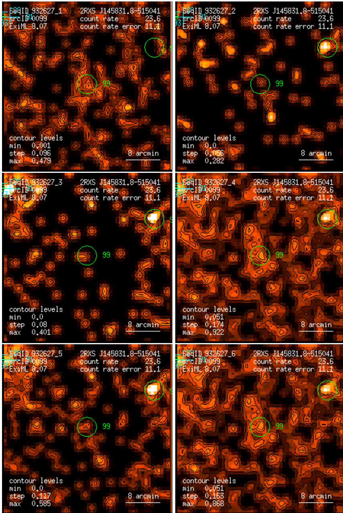
Figure 99: RASS 932627: detection 0099: band rate images, Gaussian filter: (1) PSPC channels 11 – 41, (2) 52 – 90, (3) 91 – 201, (4) 11 – 235, (5) 52 – 201, (6) 11 – 201. Broad band rates in counts/ks. Band rate contour levels in counts/ks/arcmin 2 .
